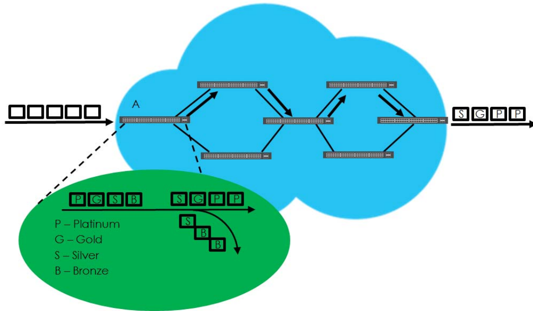
Figure 161 DiffServ Network
