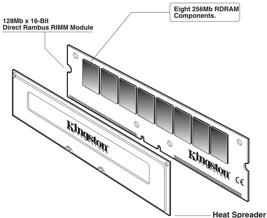
Direct Rambus RIMM Module Assembly
