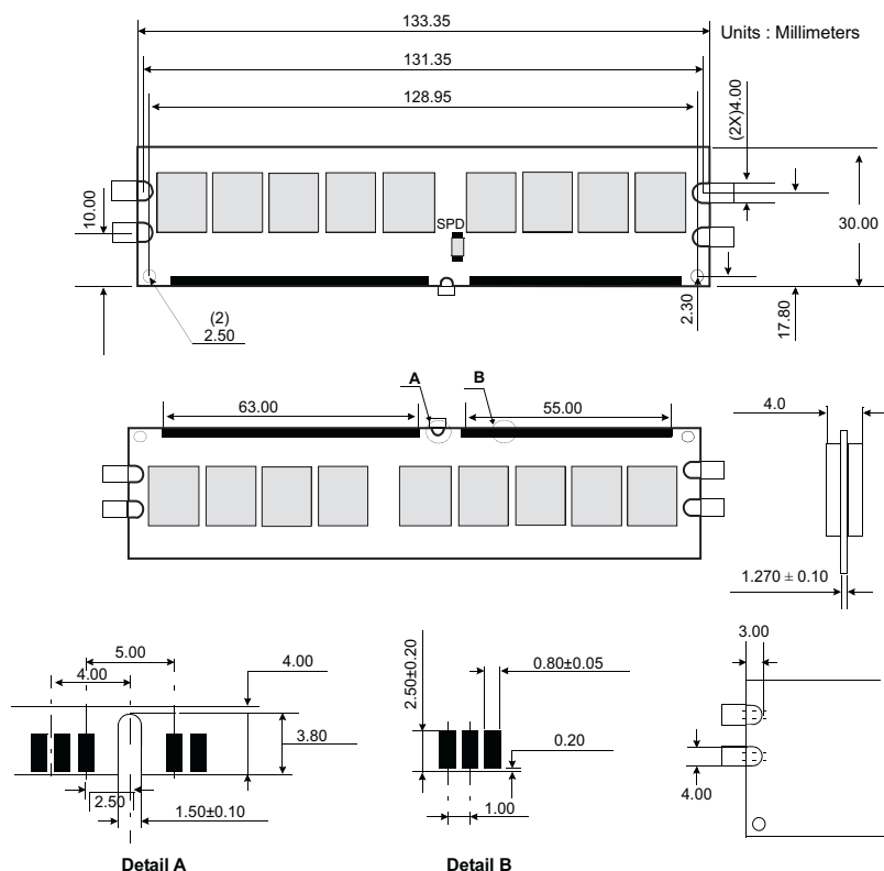
Figure 1: KVR533D2E4/2GI 240-Pin DIMM
