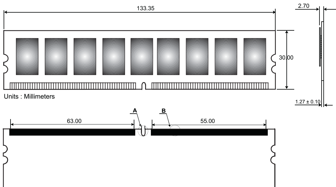
Figure 1: KVR400D2E3K2/1G 240-Pin DIMM
