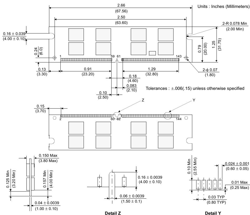
Figure 1: KVR133X64SC3L/512 144-Pin SDRAM Module
