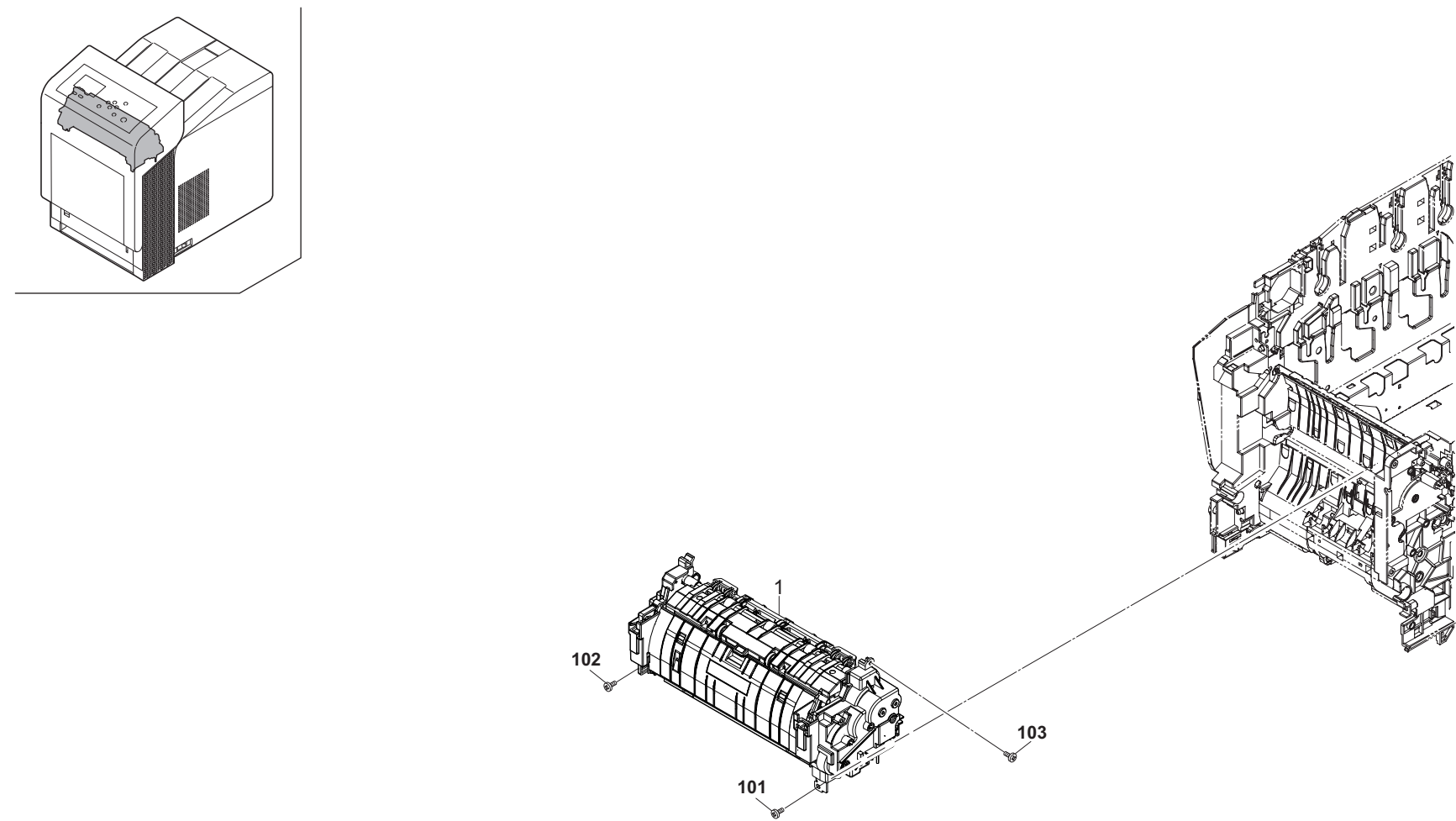
FIG. 11 Fuser Section
