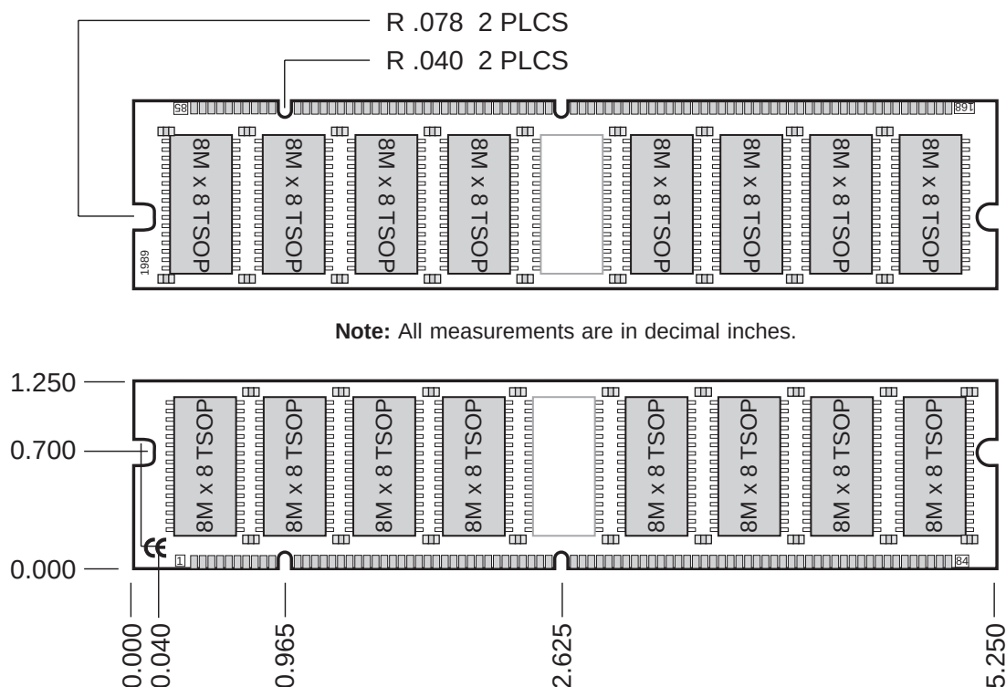
Figure 1: KVR66X64/128 168-Pin SDRAM Module
