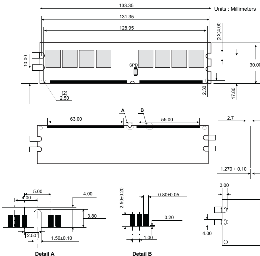
Figure 1: KVR533D2N4K2/512 240-Pin DIMM Kit
