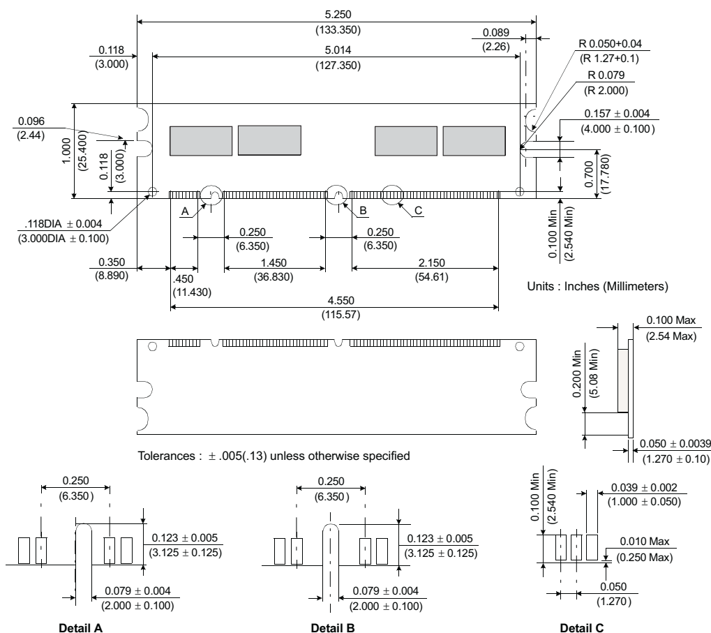
Figure 1: KVR133X64C3L/128 168-Pin SDRAM Module
