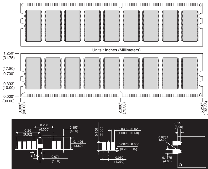
Figure 1: KVR266X72C25K8/4G 184-Pin DIMM
