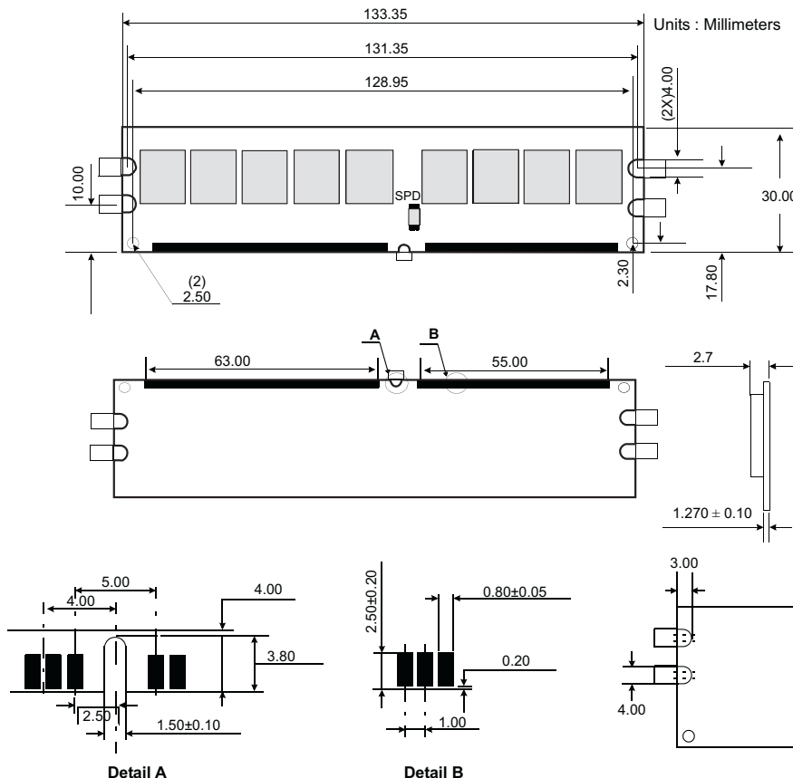
Figure 1: KVR533D2E4/512I 240-Pin DIMM
