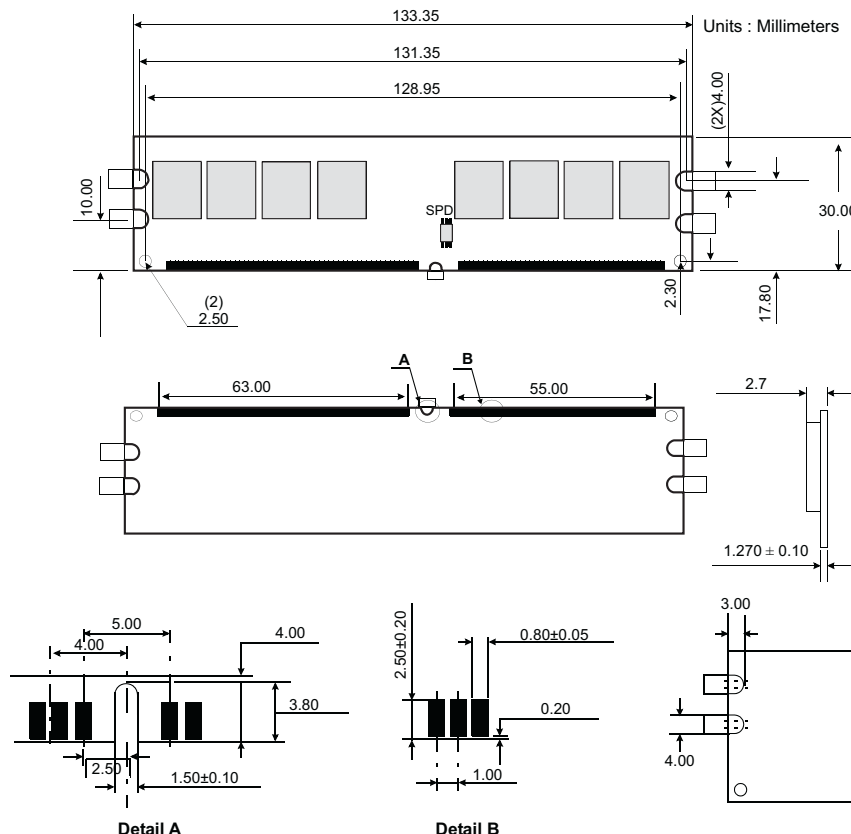
Figure 1: KVR667D2N5K2/1G 240-Pin DIMM Kit
