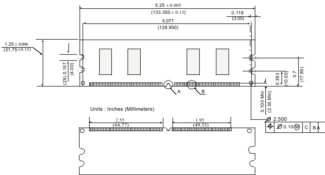
Figure 1: KVR400X64C3A/128 184-Pin DIMM
