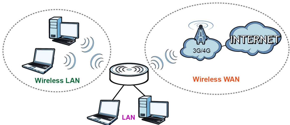
Figure 26 LAN/Wireless LAN and Wireless WAN
