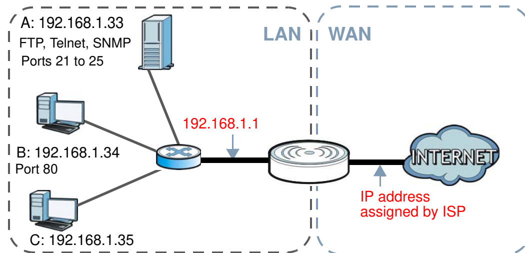
Figure 54 NAT Example
