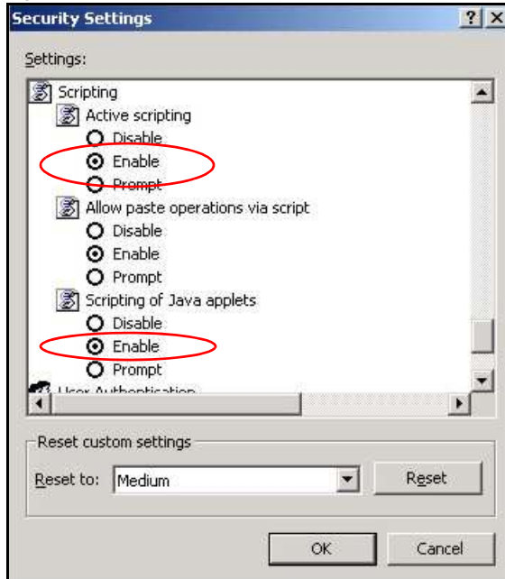
Figure 102 Security Settings - Java Scripting
