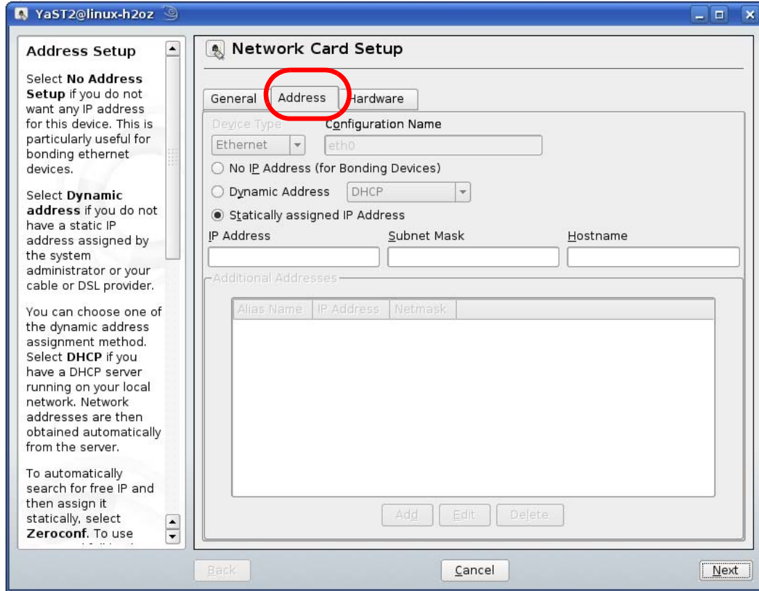
Figure 113 openSUSE 10.3: Network Card Setup
