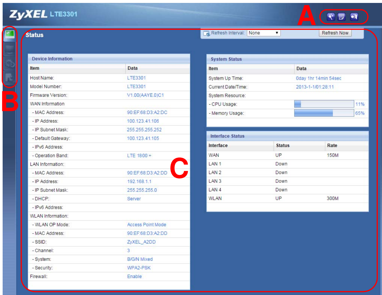
Figure 5 The Web Configurator's Main Screen
