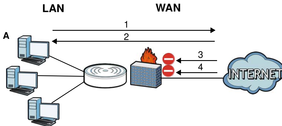
Figure 69 Default Firewall Action
