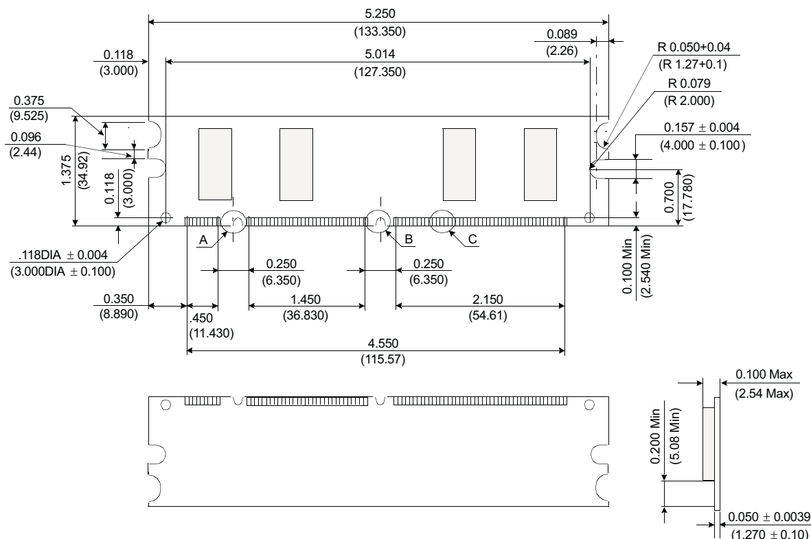
Figure 1: KVR133X64C3SS/128 168-Pin SDRAM Module
