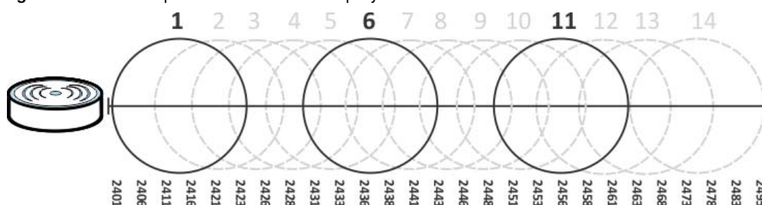
Figure 48 An Example Three-Channel Deployment
