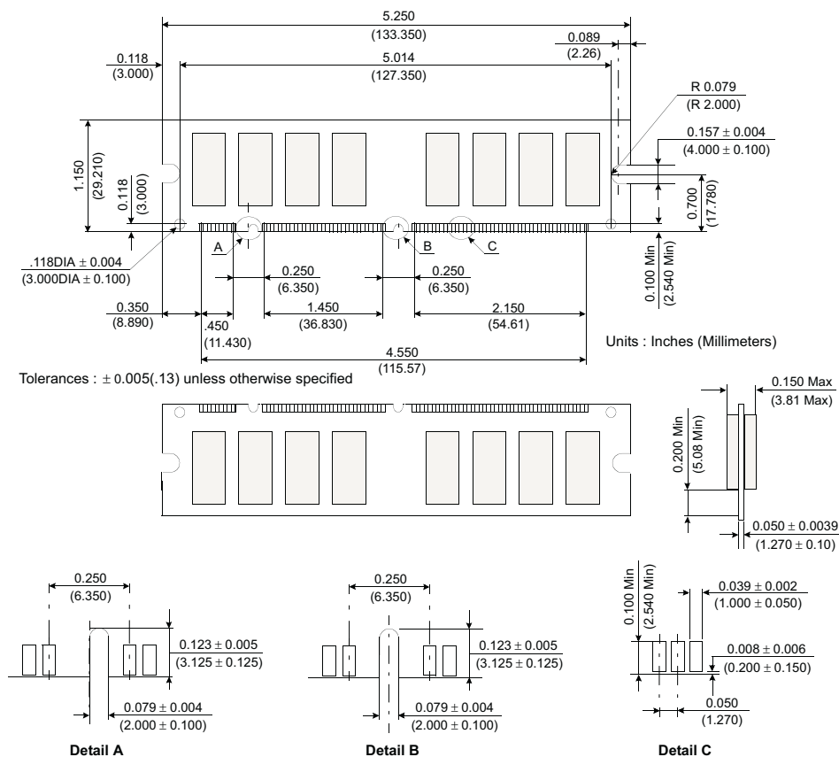
Figure 1: KVR133X64C3L/512 168-Pin SDRAM Module
