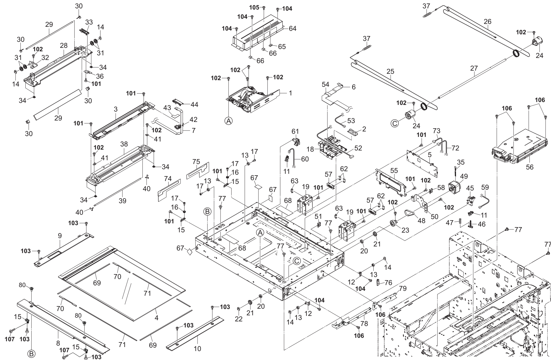
FIG. 19 Scanner & Laser Scanner Section
