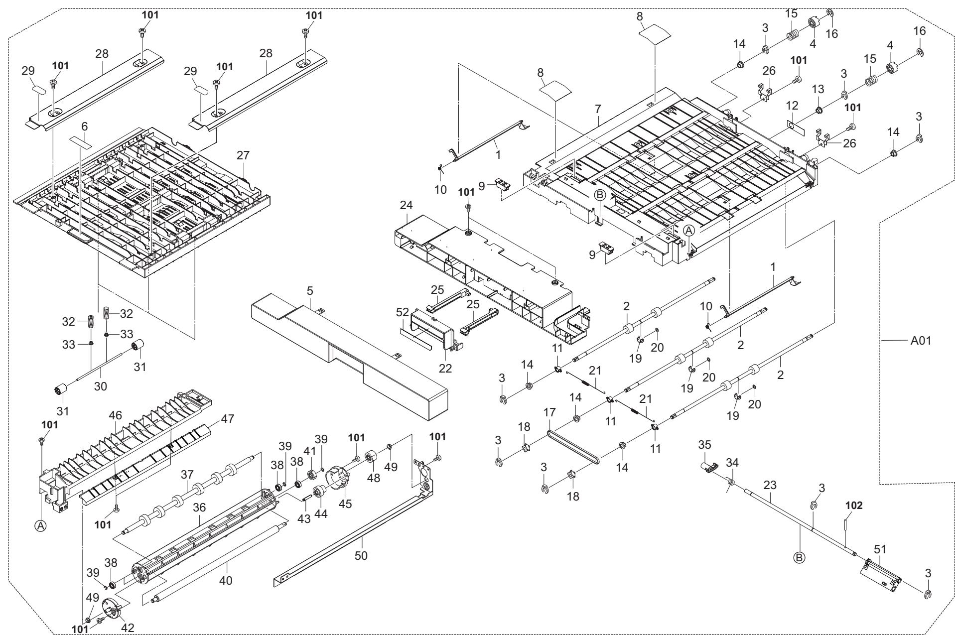
FIG. 29 Bridge Section 1
