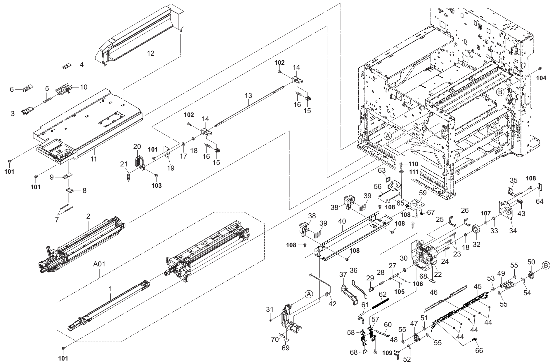
FIG. 20 Image Formation & Developer Section
