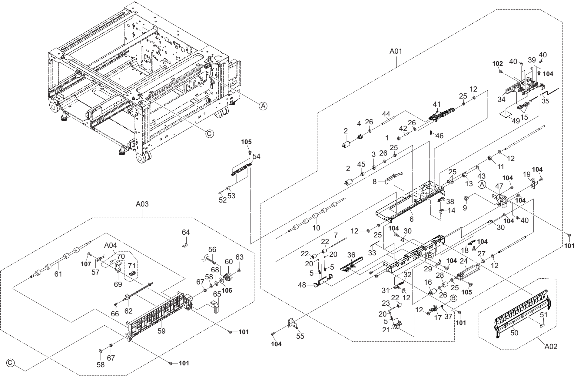
FIG. 9 Paper Deck Feed Section 1
