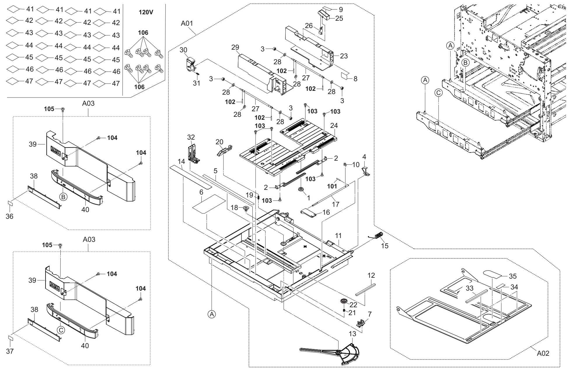
FIG. 5 Paper Cassettes
