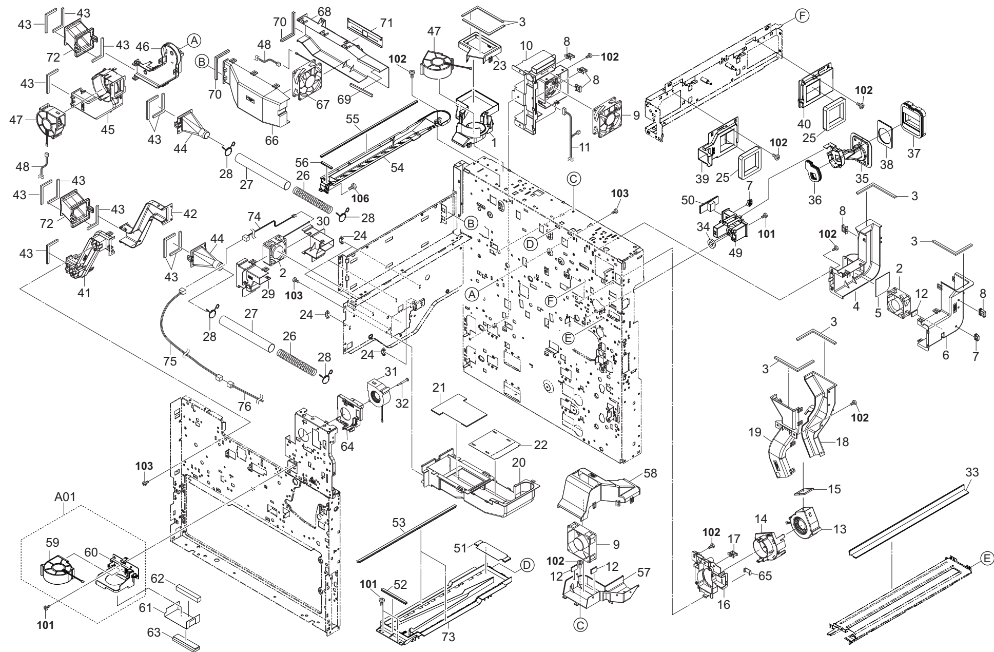
FIG. 26 Cooling Section
