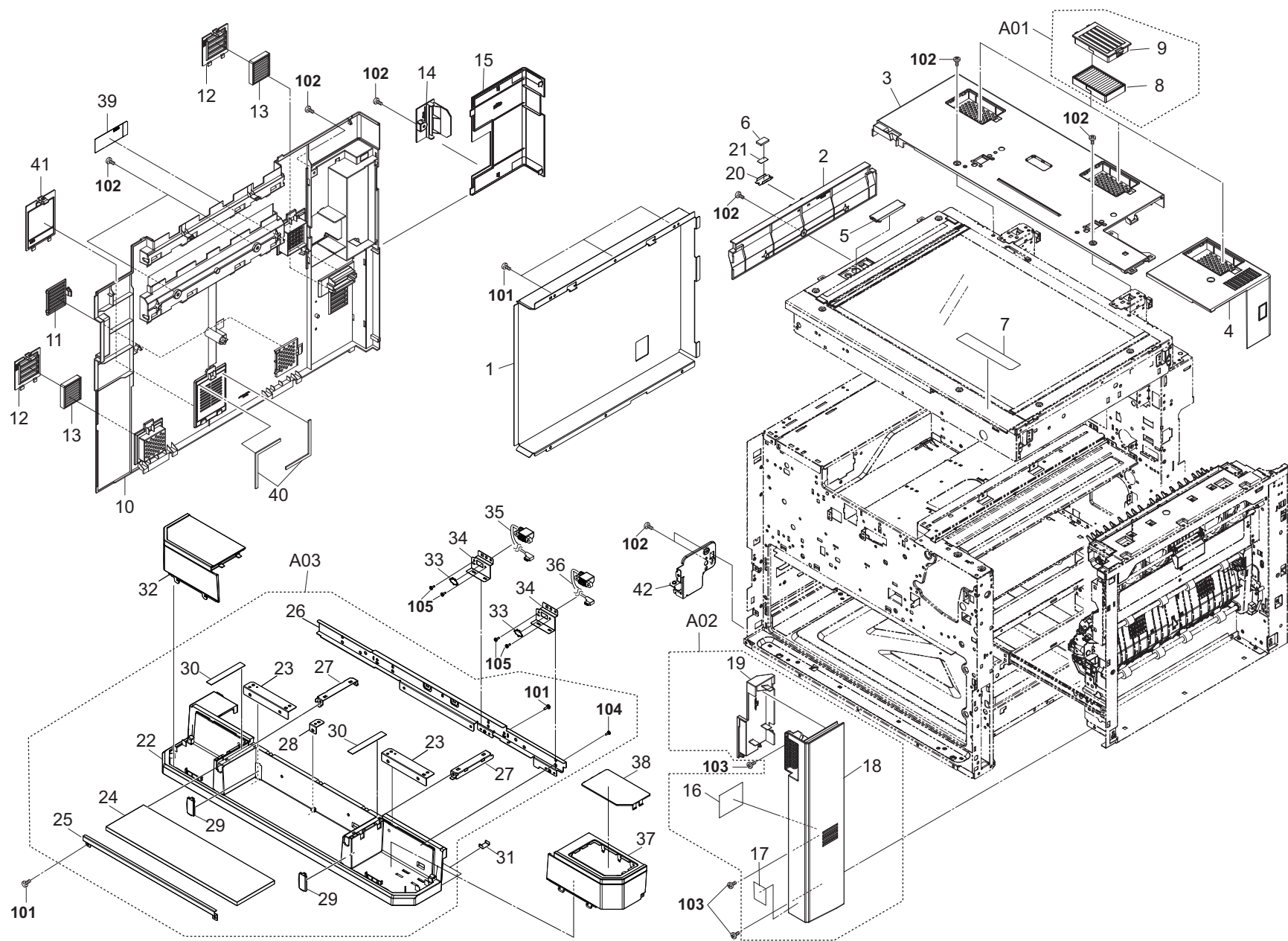
FIG. 2 Covers 2
