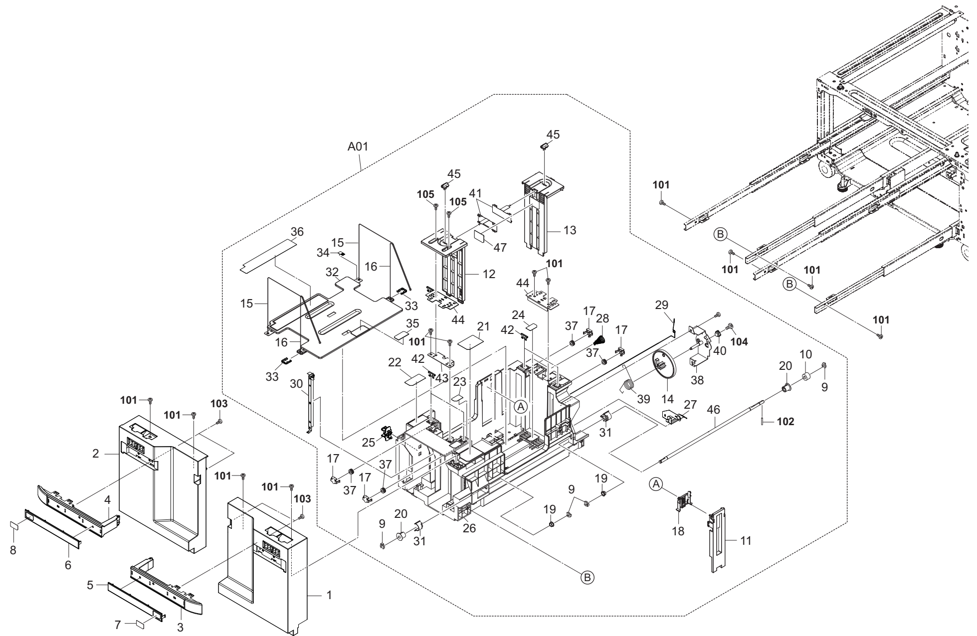
FIG. 8 Paper Deck Cassettes
