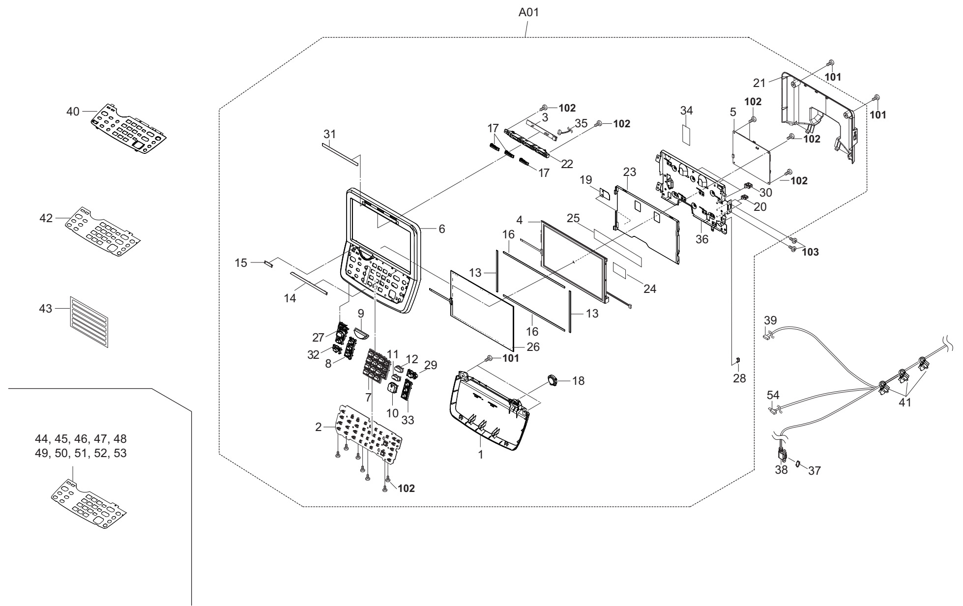
FIG. 34 Operation Panel Section
