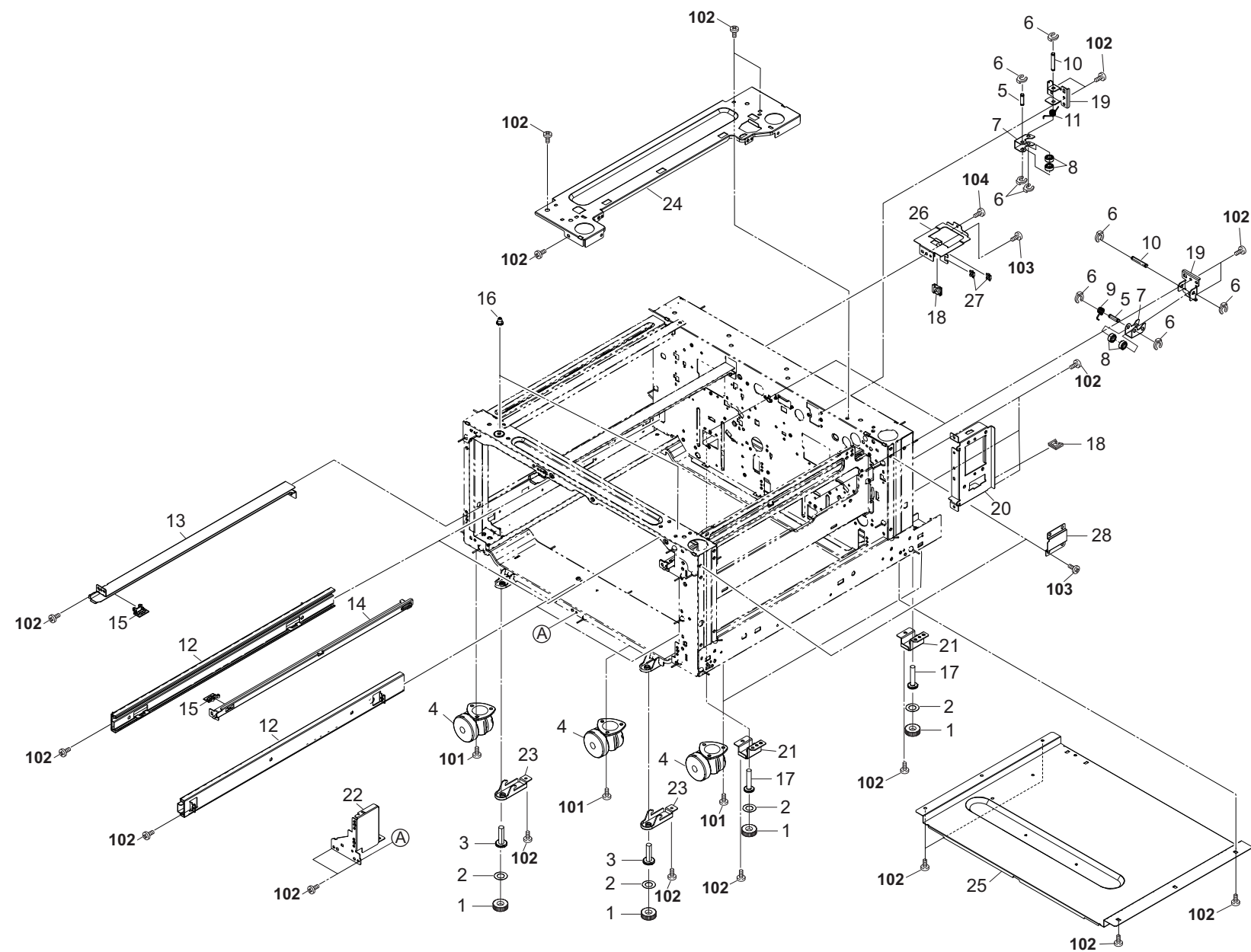
FIG. 7 Paper Deck Frames
