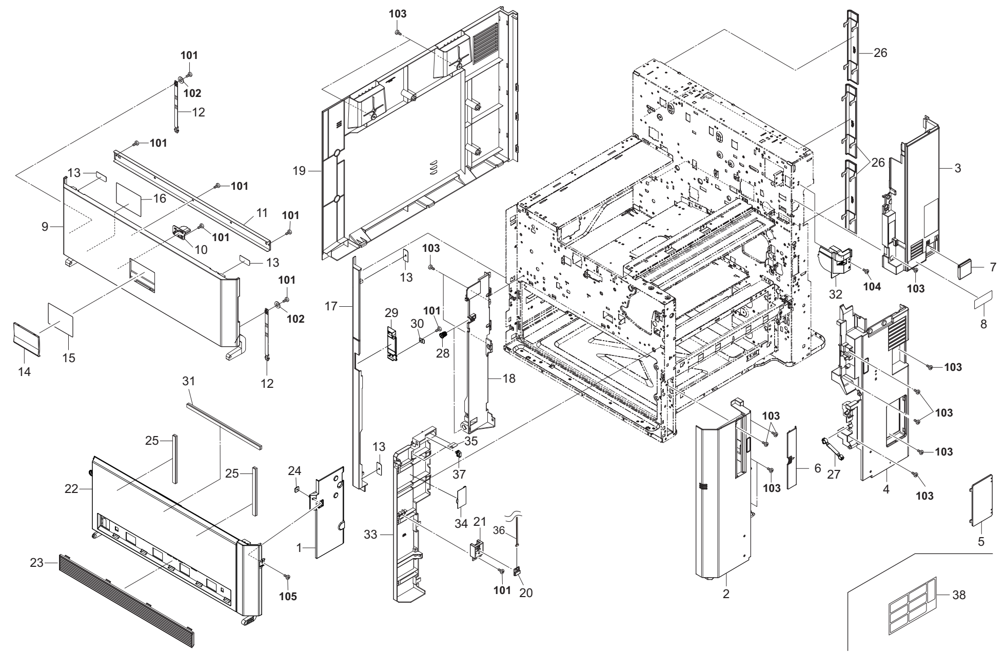
FIG. 1 Covers 1
