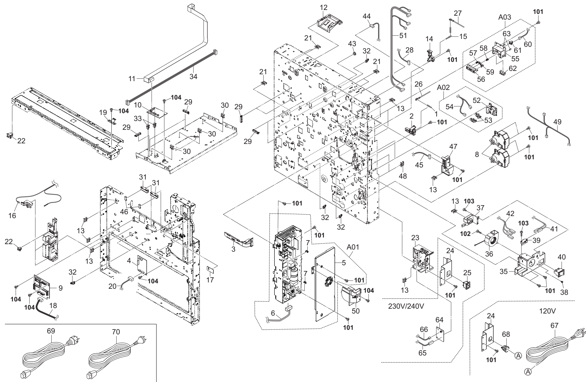
FIG. 32 Electrical Components 1
