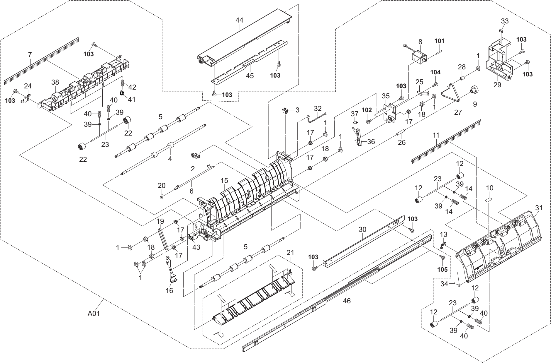
FIG. 31 Bridge Section 3
