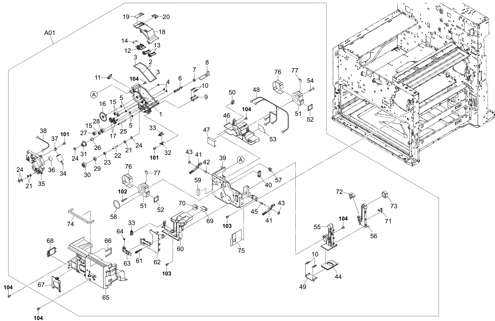
FIG. 21 Inner Section 1
