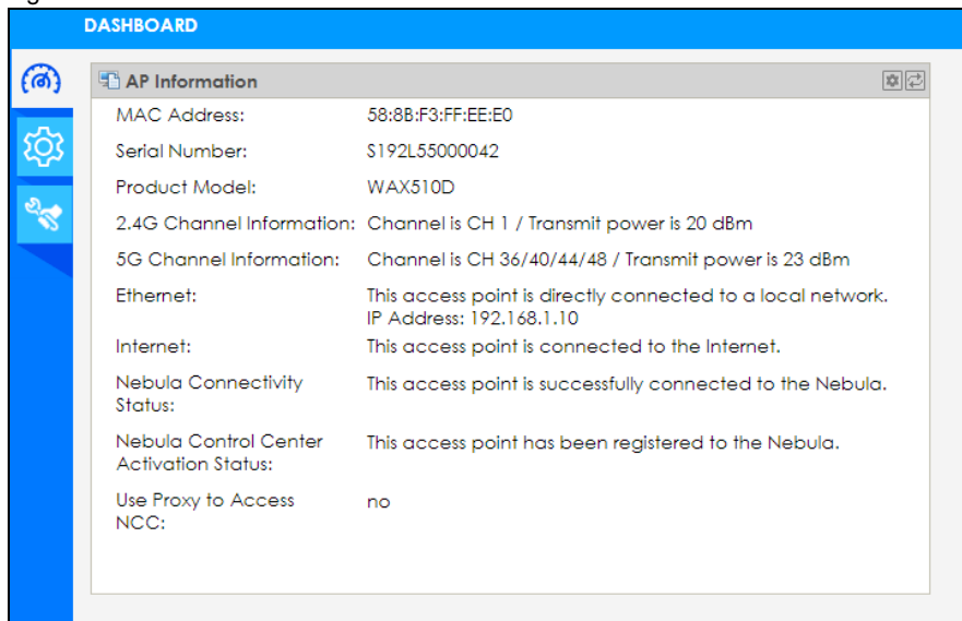
Figure 141 Dashboard
