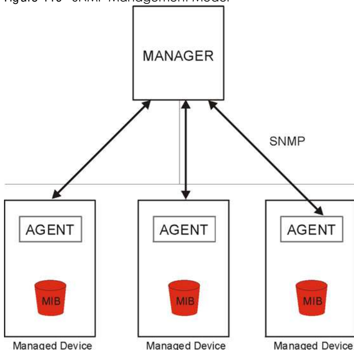
Figure 119 SNMP Management Model
