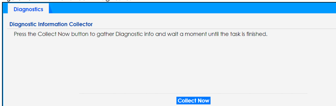
Figure 132 Maintenance > Diagnostics
