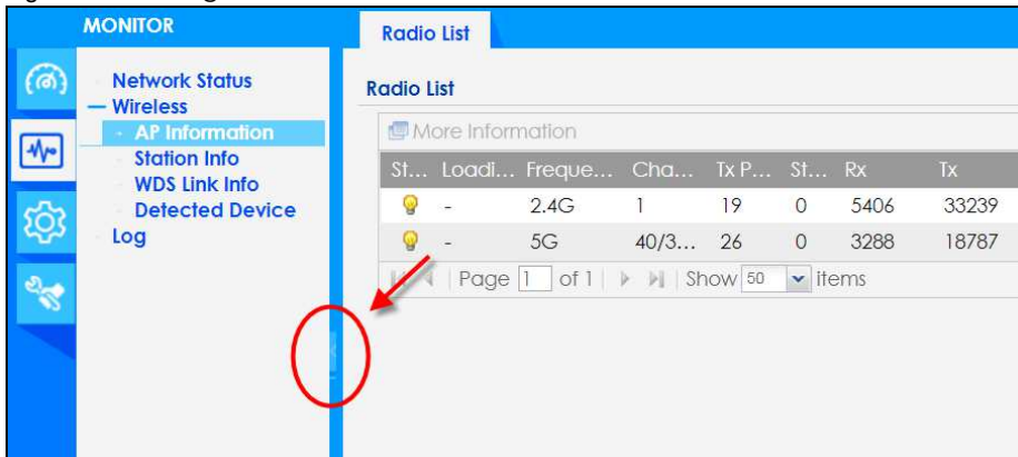
Figure 28 Navigation Panel
