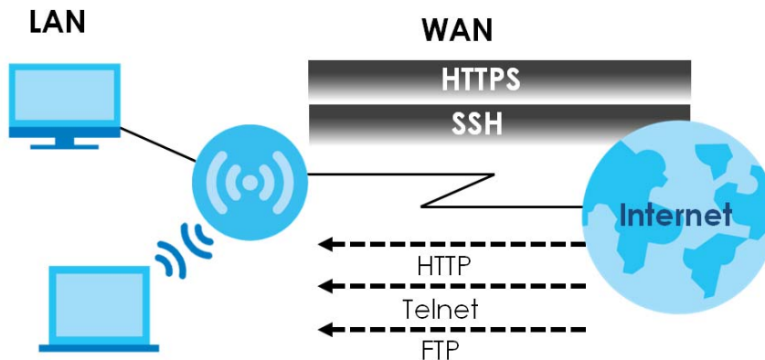
Figure 105 Secure and Insecure Service Access From the WAN
