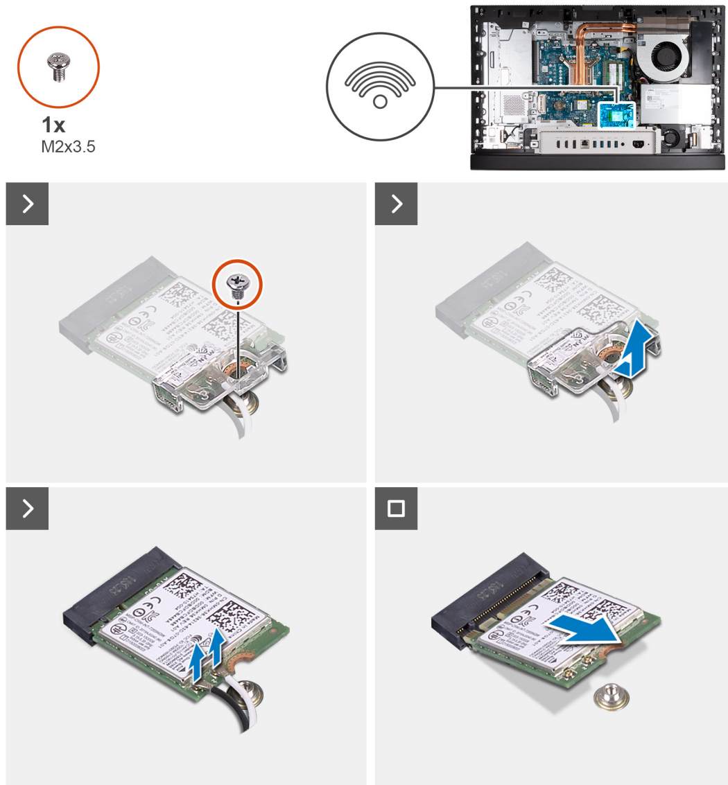
Figure 28. Removing the wireless card
