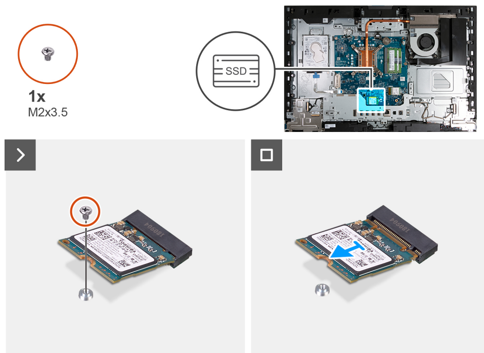
Figure 90. Removing the M.2 2230 solid-state drive
