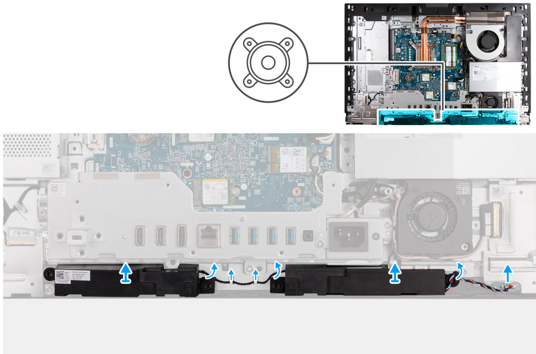
Figure 60. Removing the speakers
