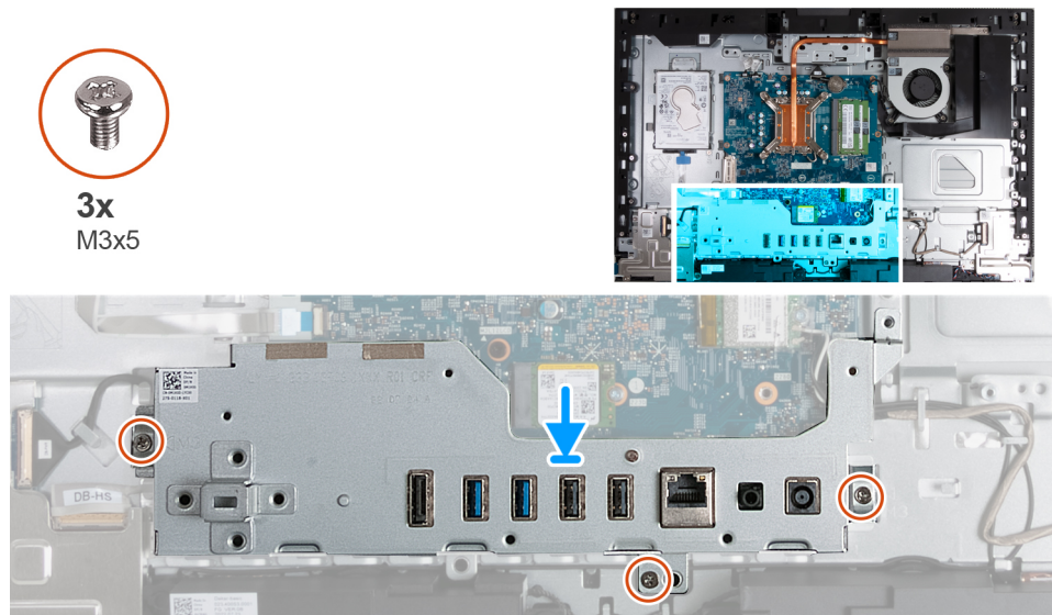
Figure 106. Installing the I/O bracket
