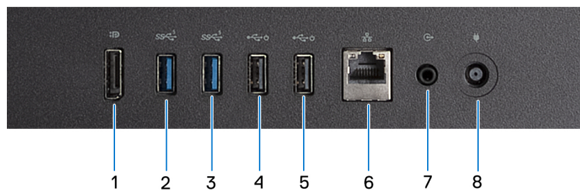
Figure 7. Back panel view of OptiPlex All-in-One 7420 with an Energy Efficient processor
