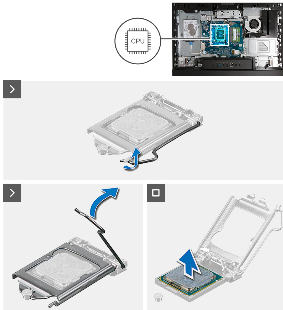
Figure 111. Removing the processor
