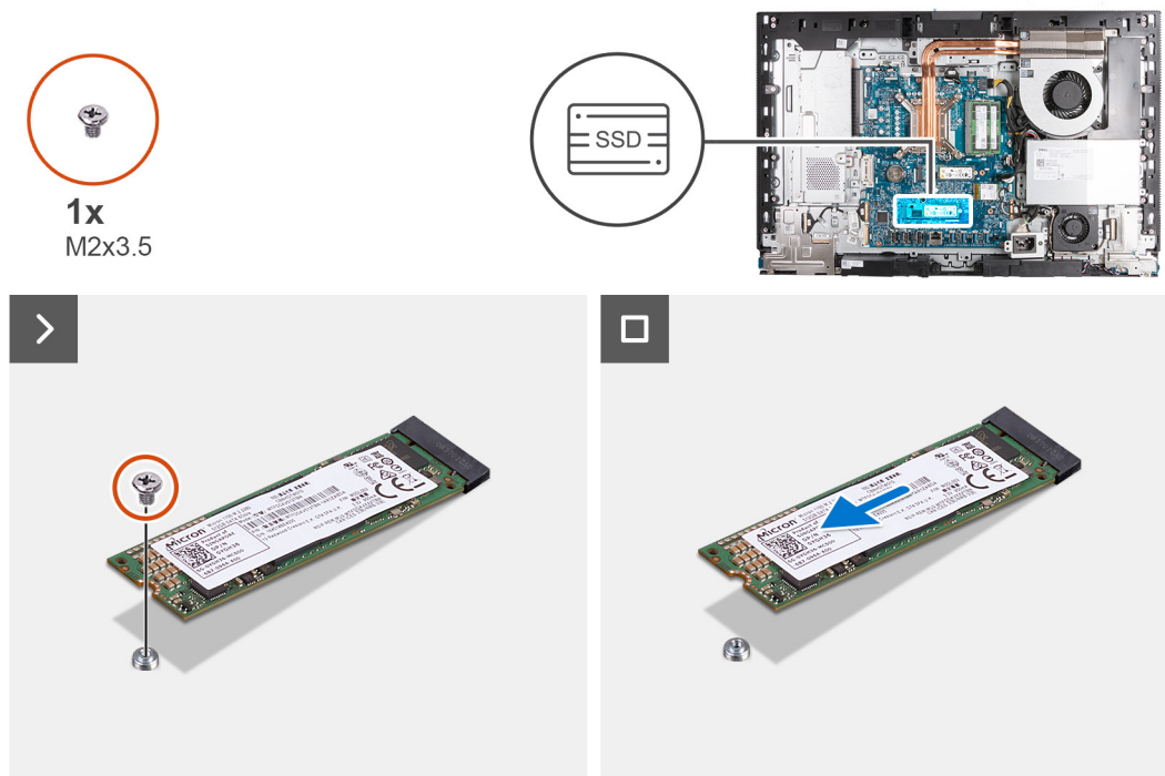
Figure 37. Removing the M.2 2280 solid-state drive in M.2 slot 1
