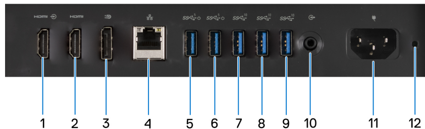
Figure 8. Back panel view of OptiPlex All-in-One 7420 with a High Performance processor
