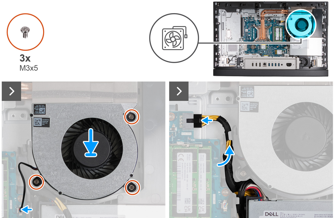
Figure 49. Installing the fan
