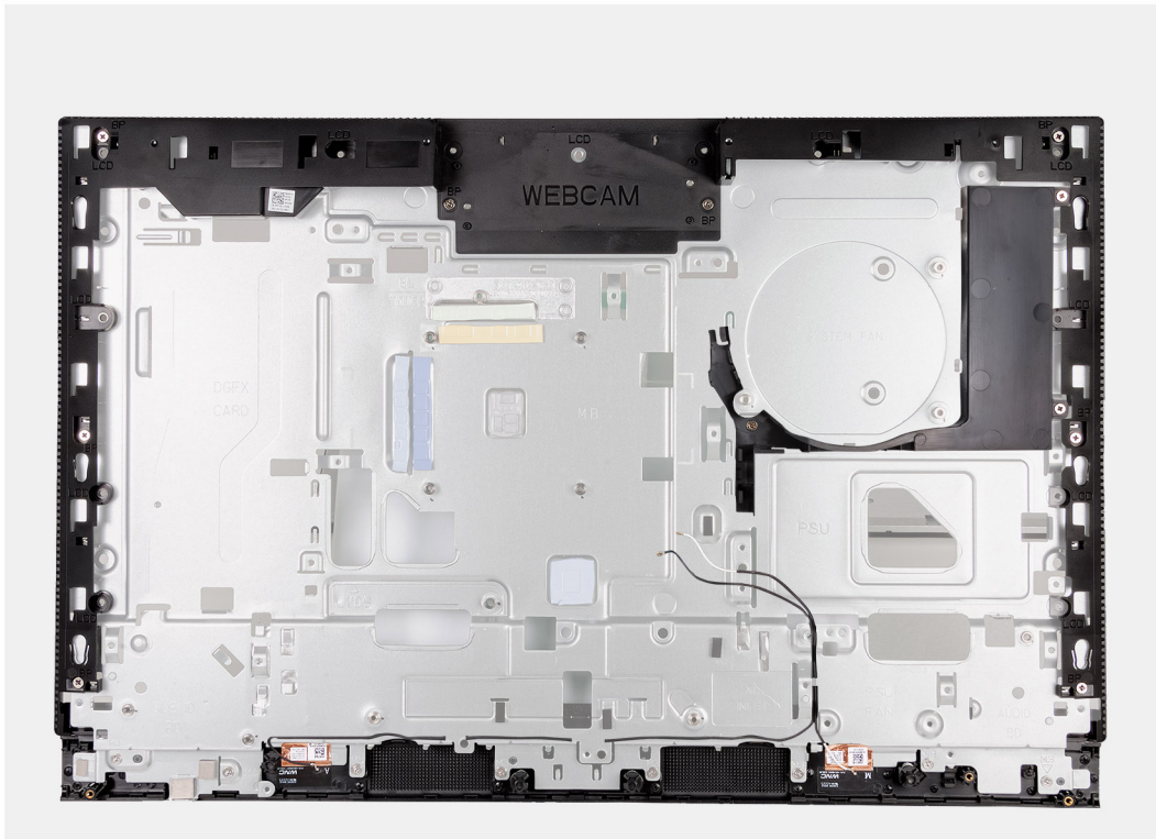
Figure 77. Installing the display-assembly base
