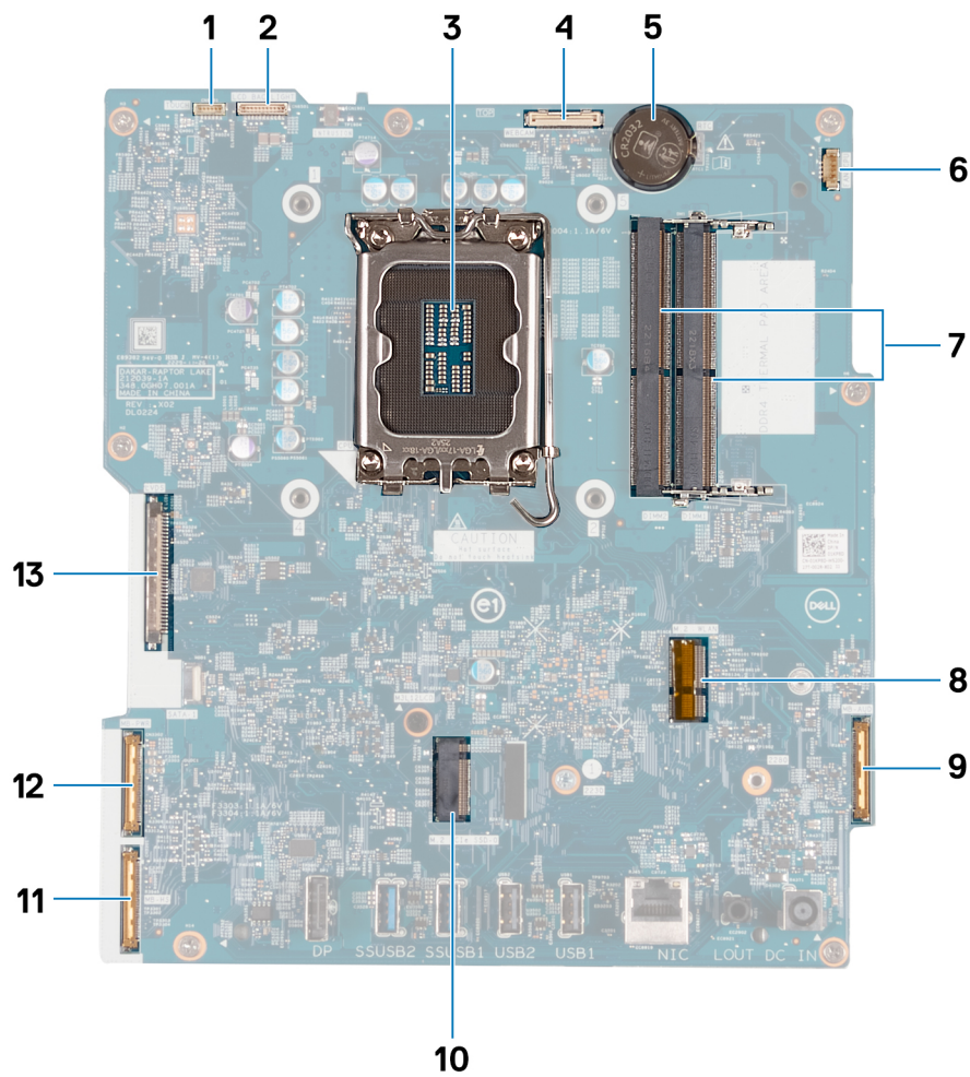
Figure 116. System board callouts
