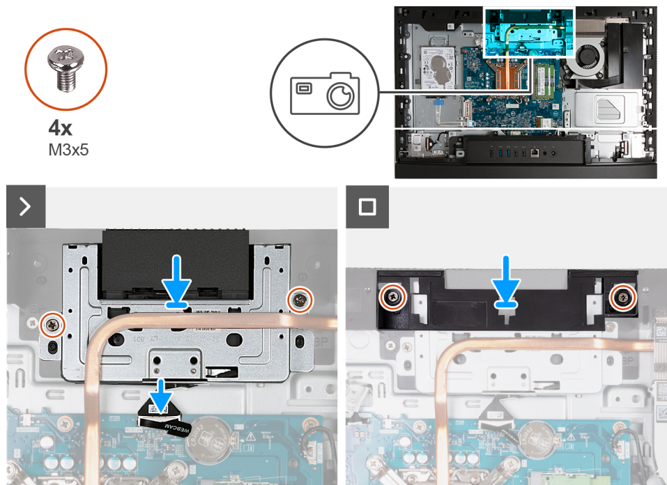
Figure 102. Installing the retractable-camera assembly
