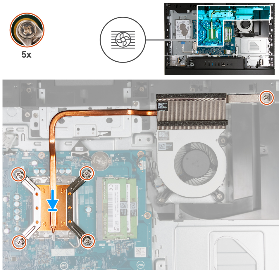
Figure 110. Installing the heat sink
