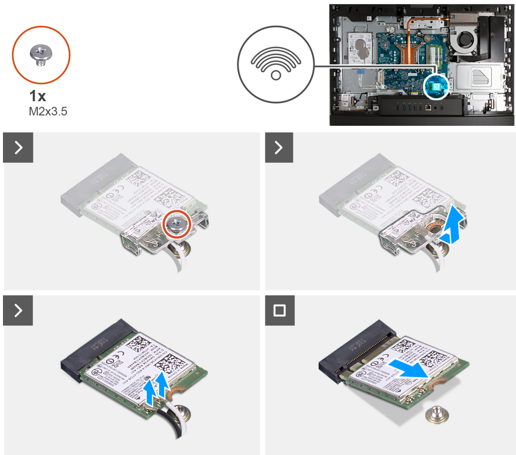
Figure 88. Removing the wireless card
