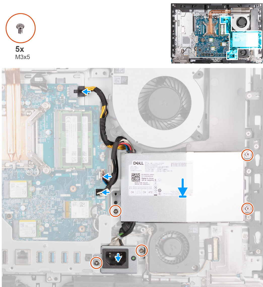
Figure 51. Installing the power-supply unit
