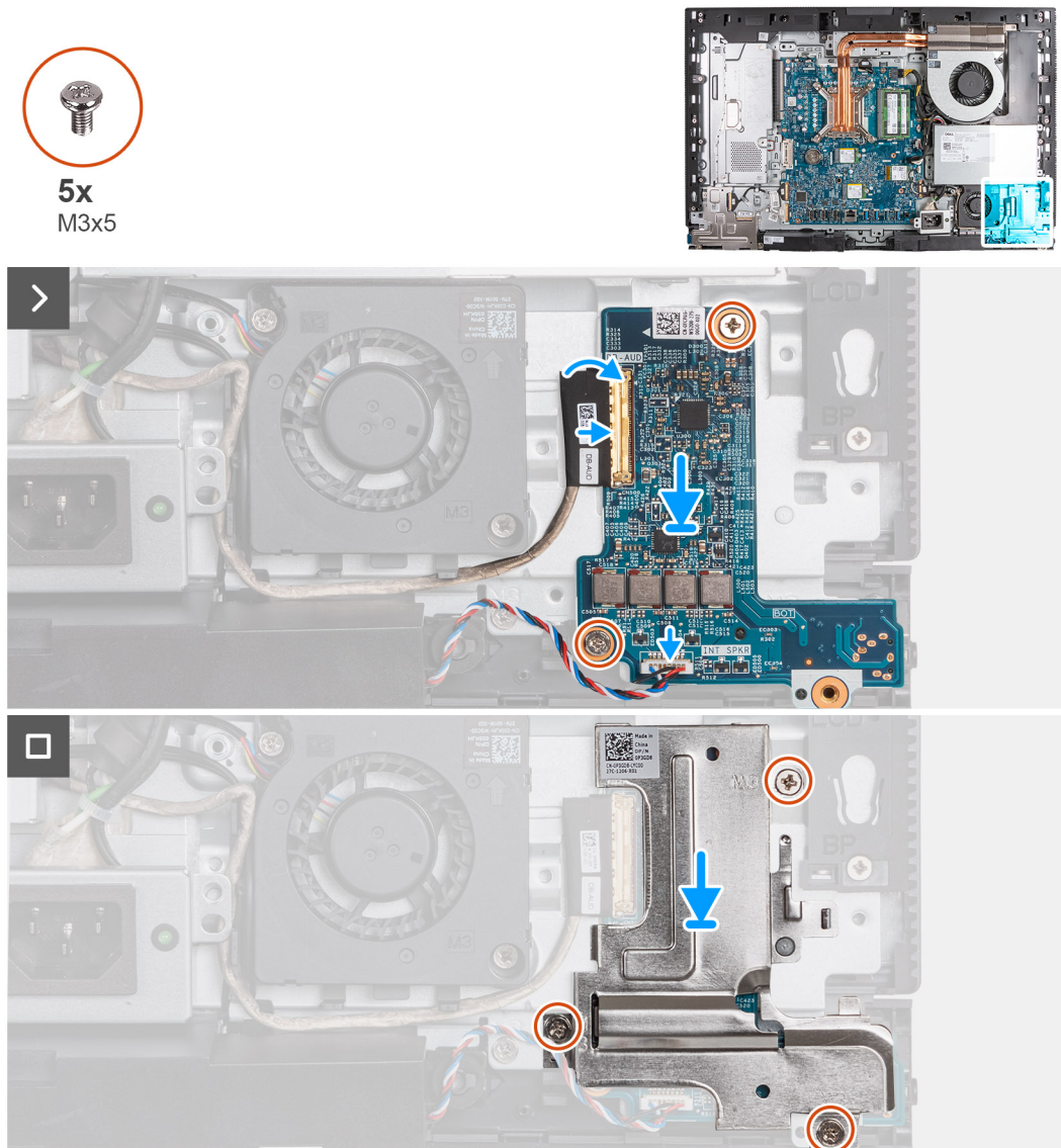
Figure 75. Installing the audio board
