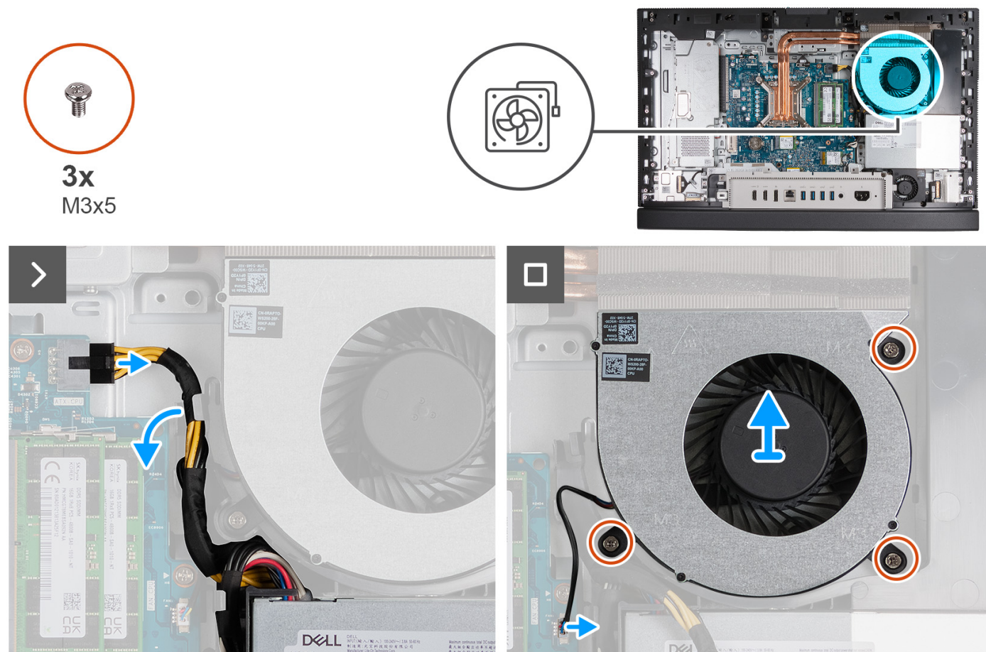
Figure 48. Removing the fan
