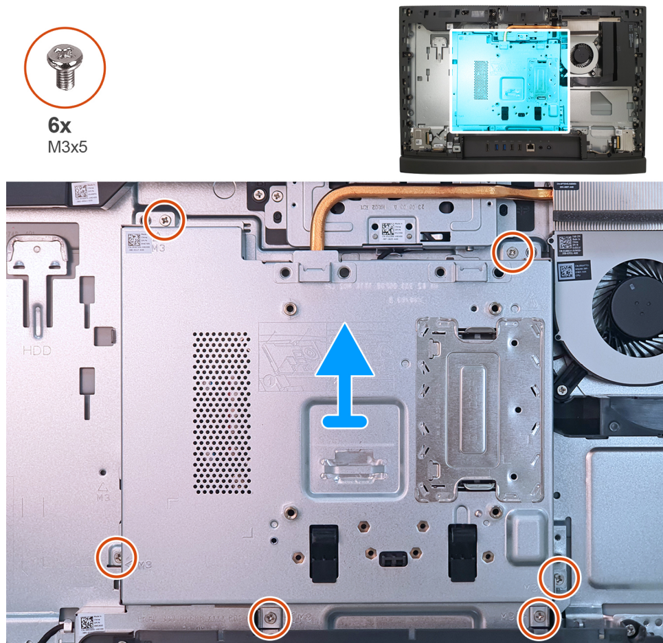
Figure 86. Removing the system-board shield
