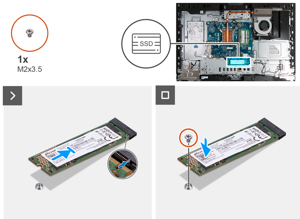
Figure 93. Installing the M.2 2280 solid-state drive
