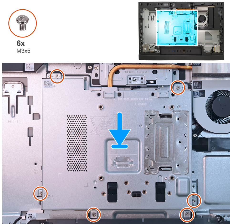
Figure 87. Installing the system-board shield
