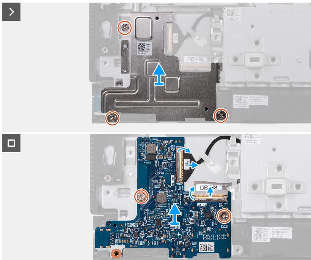
Figure 72. Removing the power-button and I/O board
