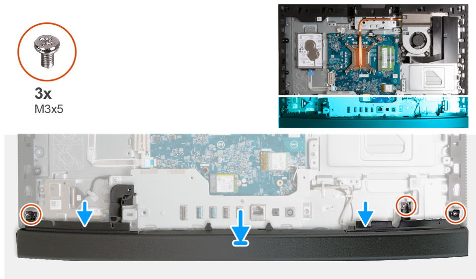
Figure 100. Installing the bottom cover
