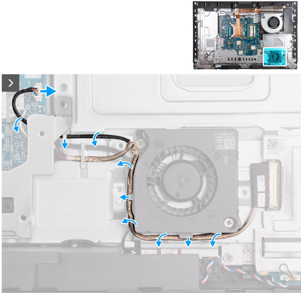
Figure 52. Removing the power-supply fan
