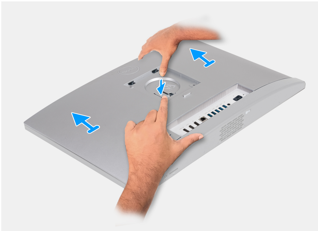
Figure 22. Removing the back cover
