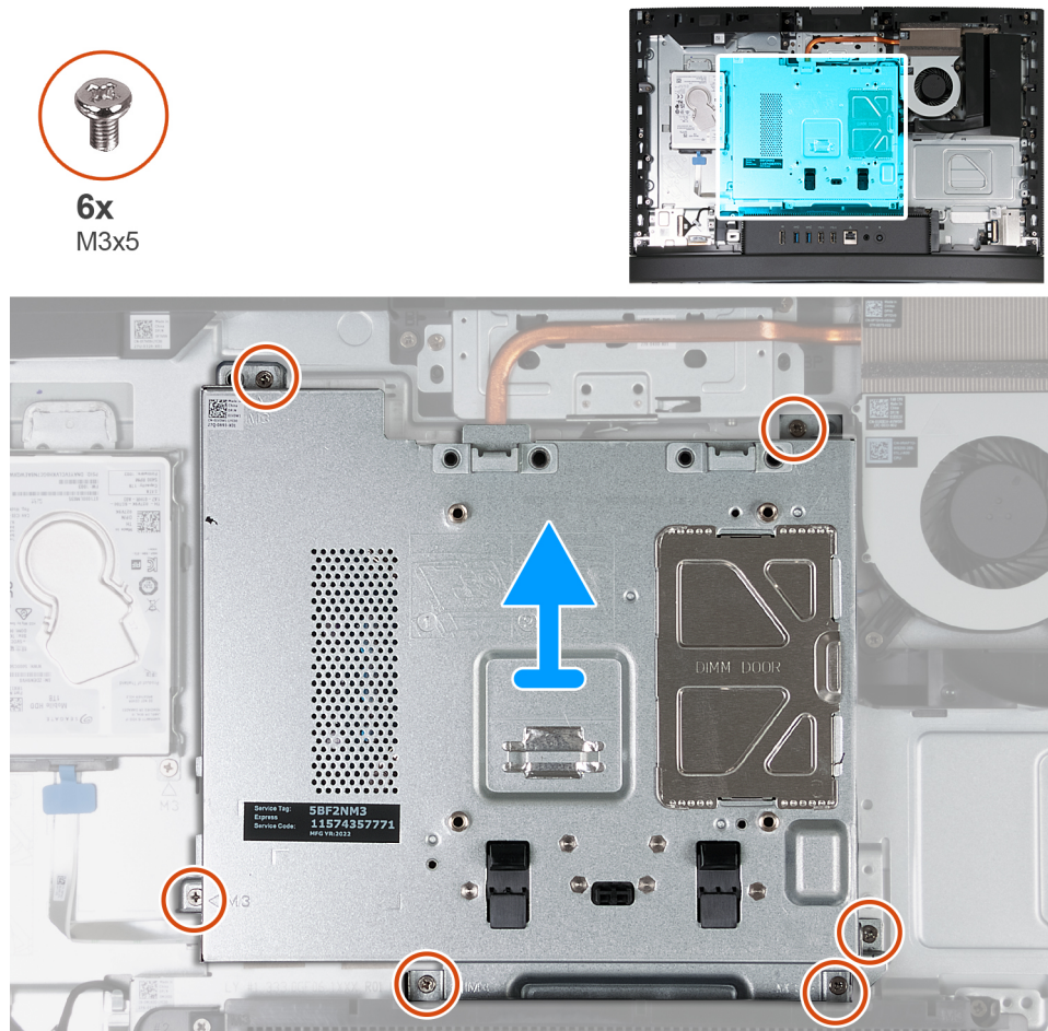
Figure 26. Removing the system-board shield
