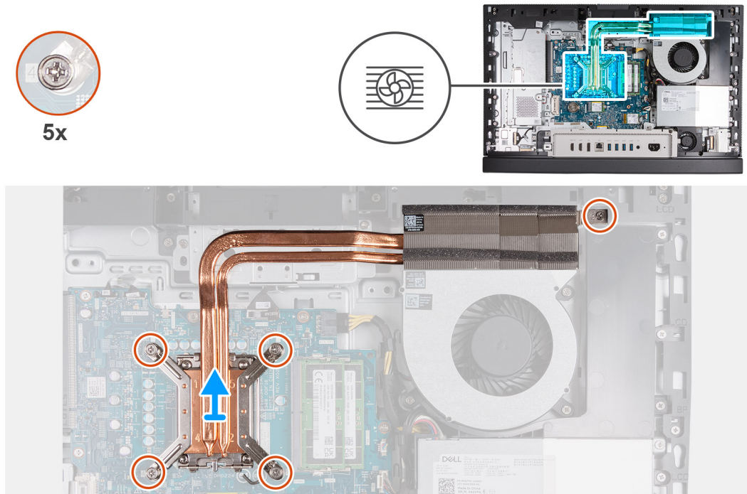
Figure 62. Removing the heat sink
