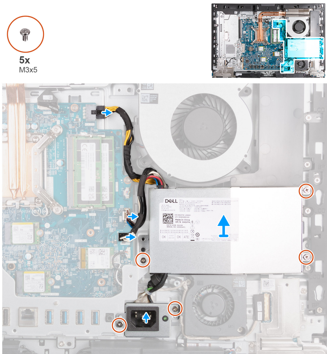
Figure 50. Removing the power-supply unit
