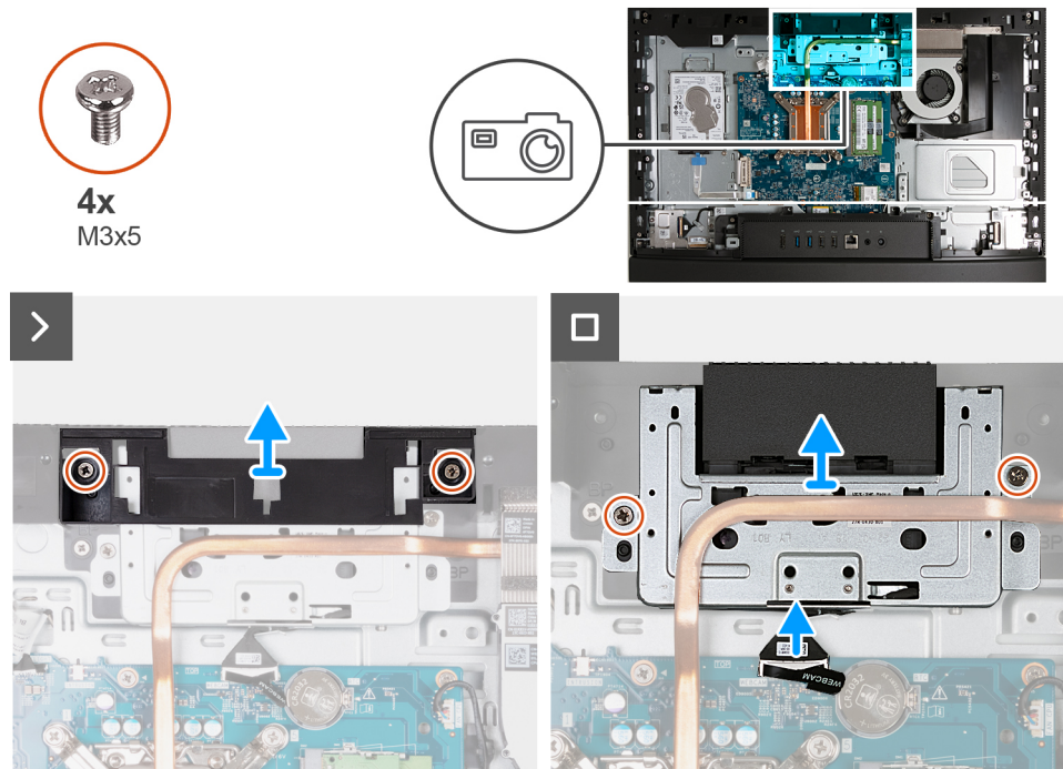
Figure 101. Removing the retractable-camera assembly
