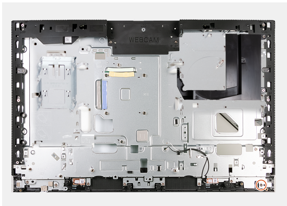
Figure 123. Removing the display-assembly base
