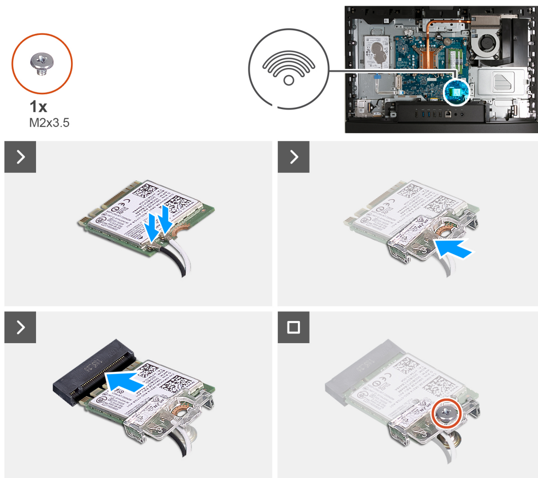
Figure 89. Installing the wireless card
