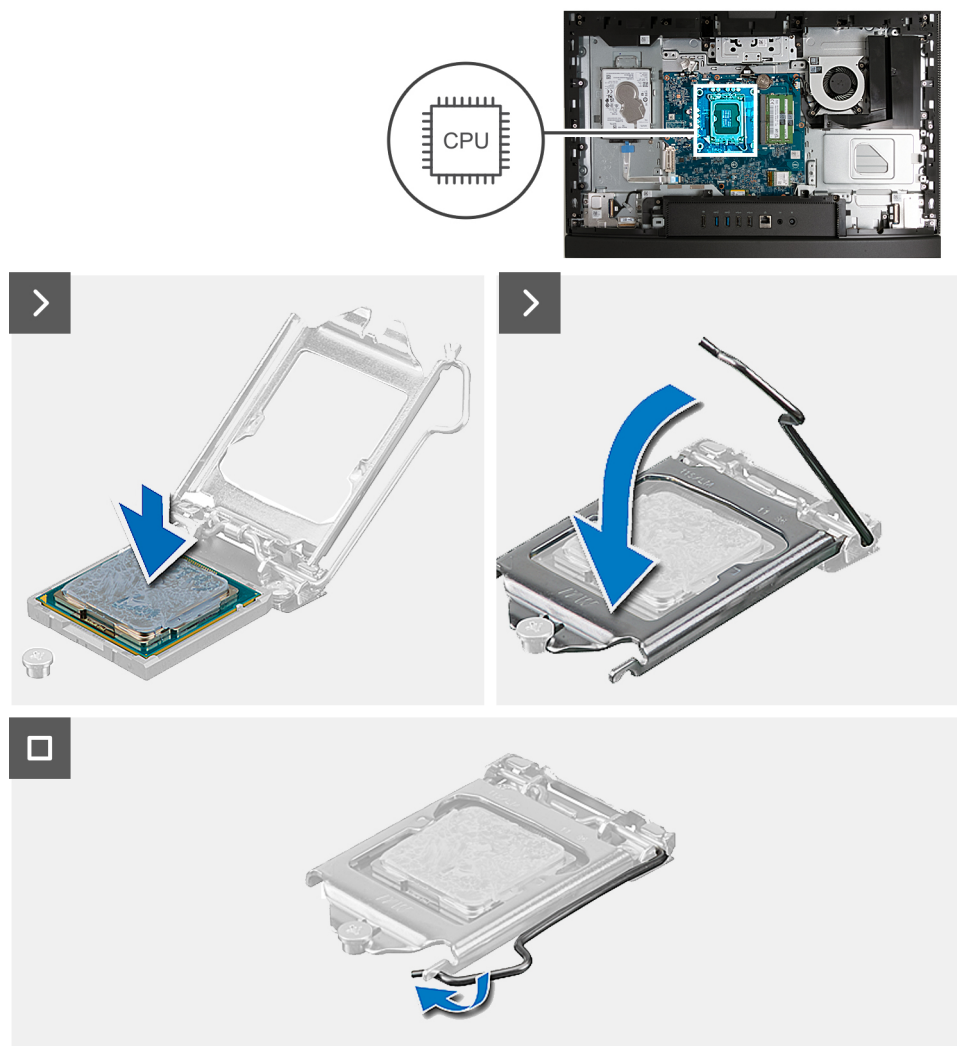
Figure 112. Installing the processor
