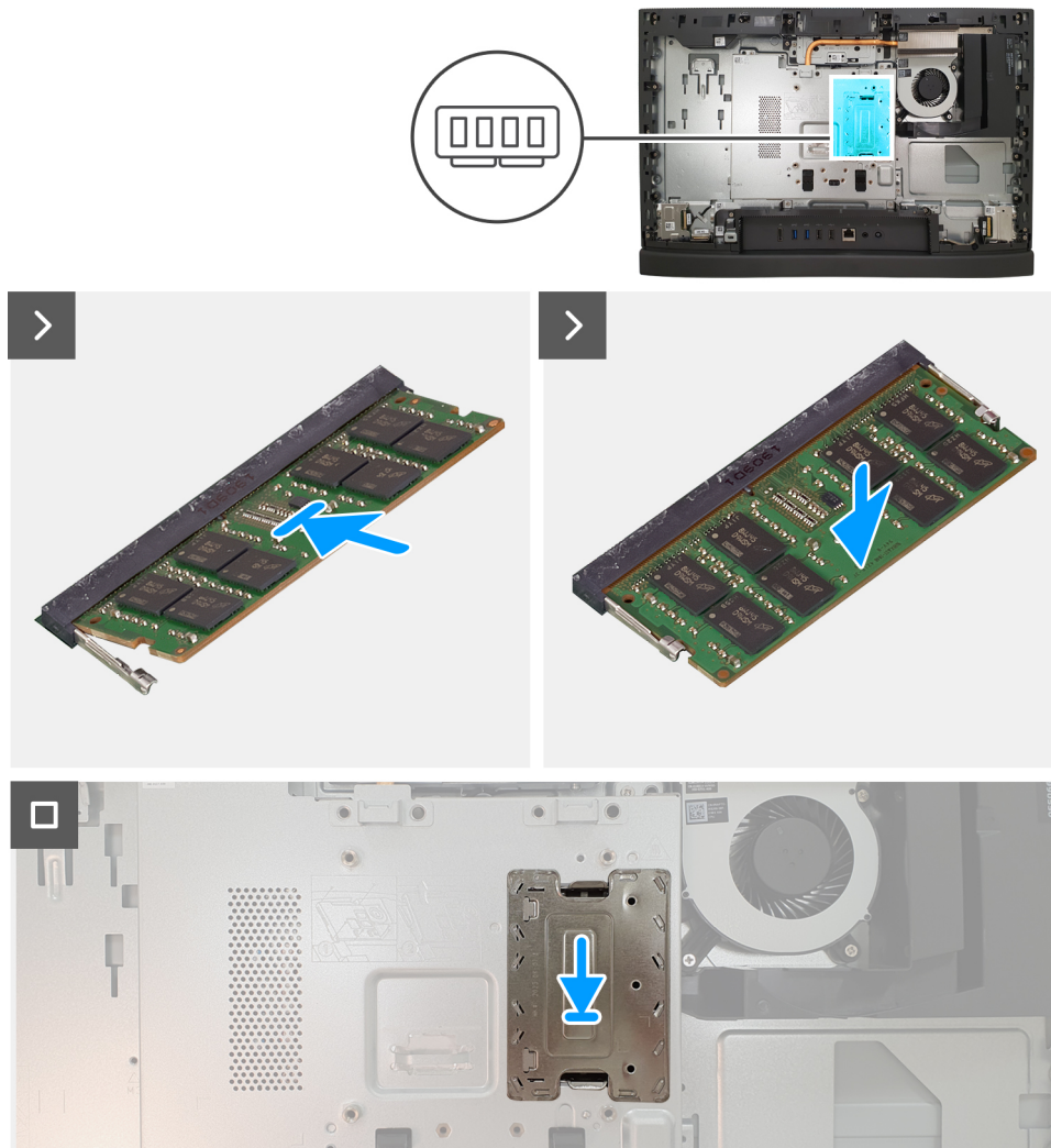
Figure 85. Installing the memory
