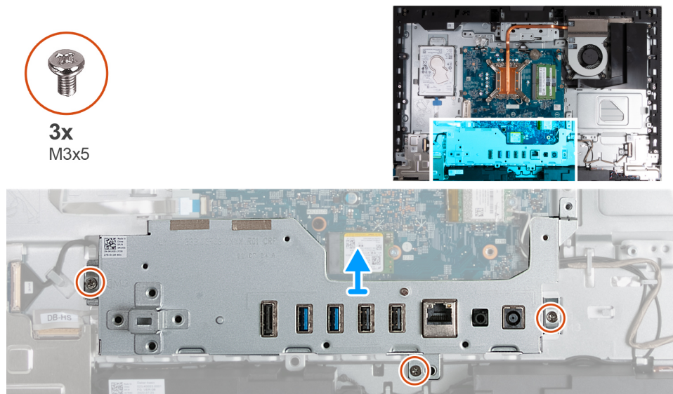
Figure 105. Removing the I/O bracket
