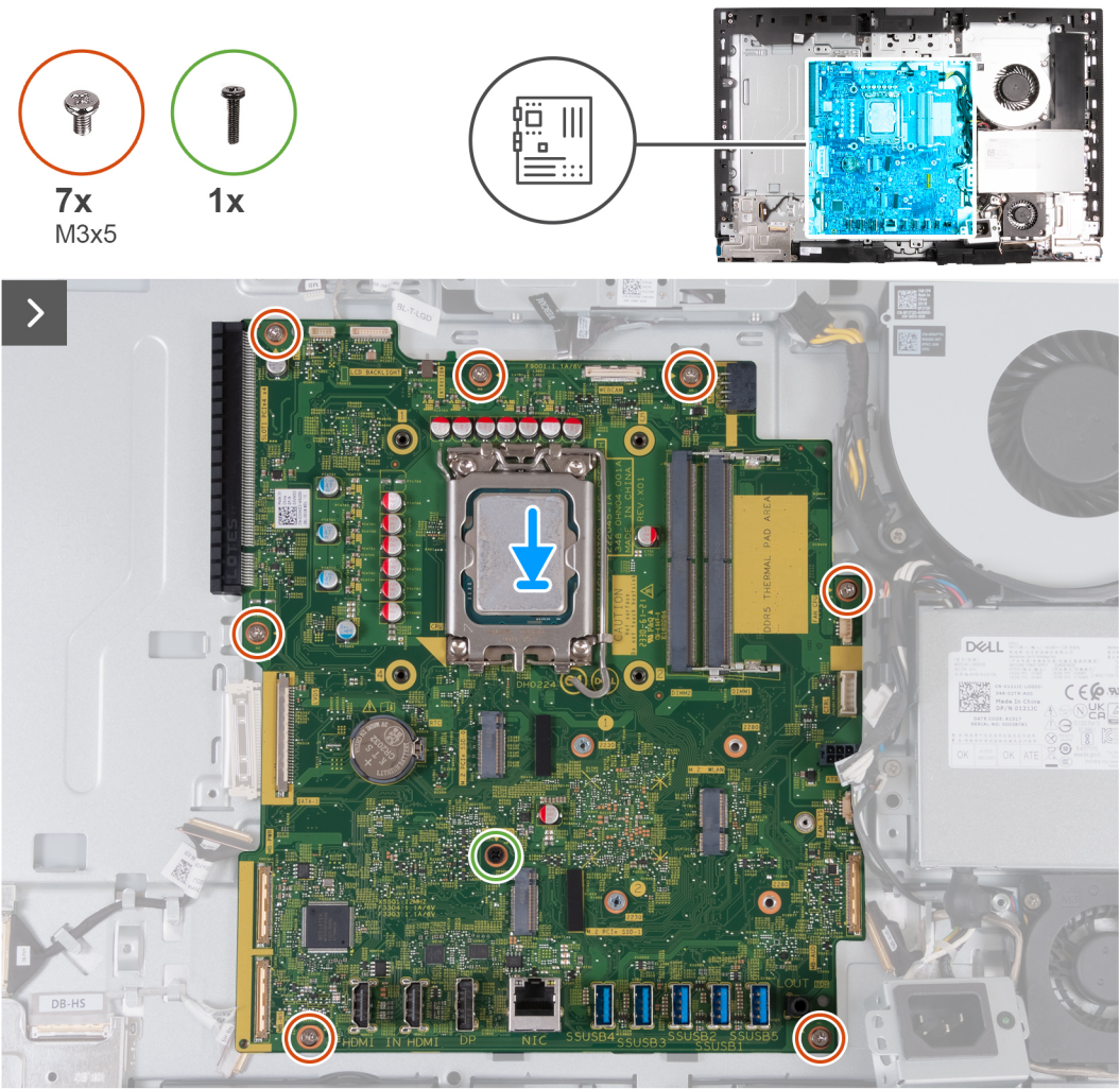
Figure 70. Installing the system board
