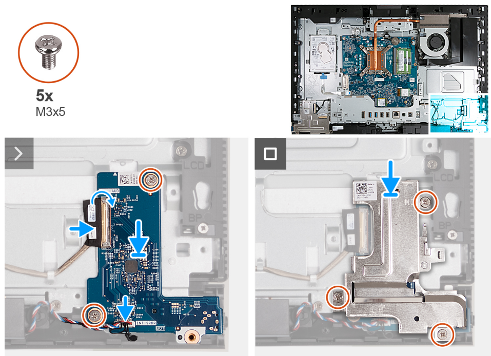
Figure 122. Installing the audio board
