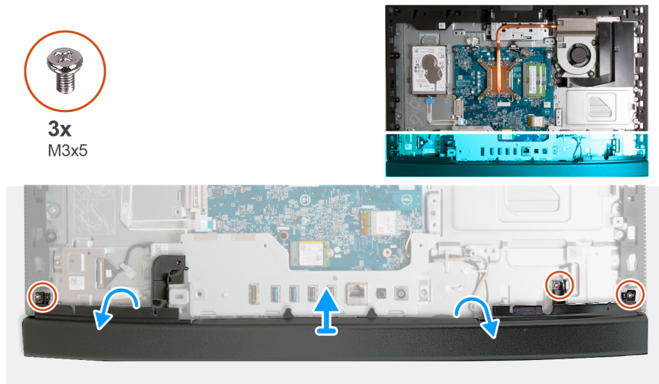
Figure 99. Removing the bottom cover
