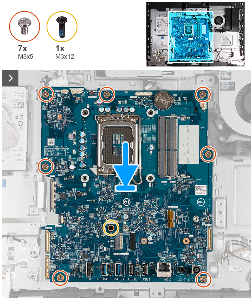
Figure 117. Installing the system board
