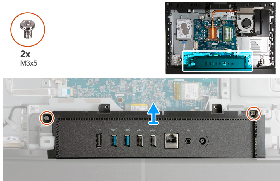
Figure 97. Removing the IO cover
