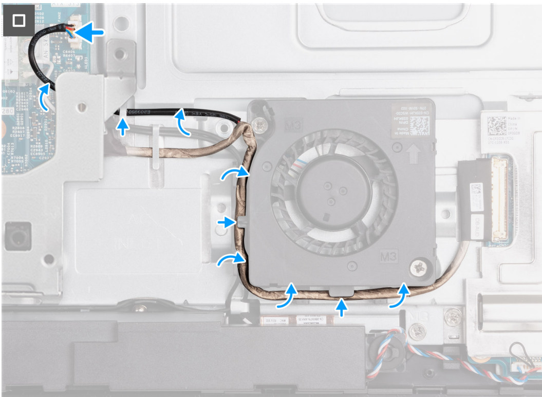
Figure 57. Installing the power-supply fan
