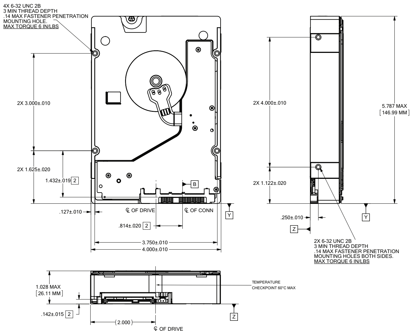
Figure 5. Mounting configuration dimensions (8TB & 6TB models)
