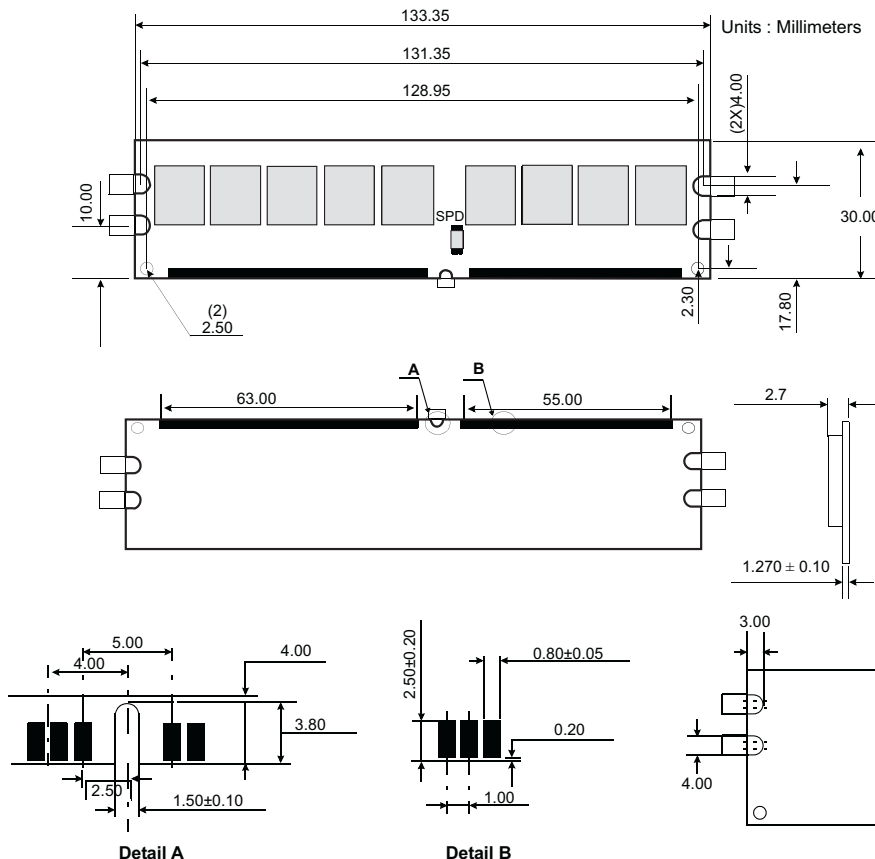
Figure 1: KVR533D2E4/512 240-Pin DIMM
