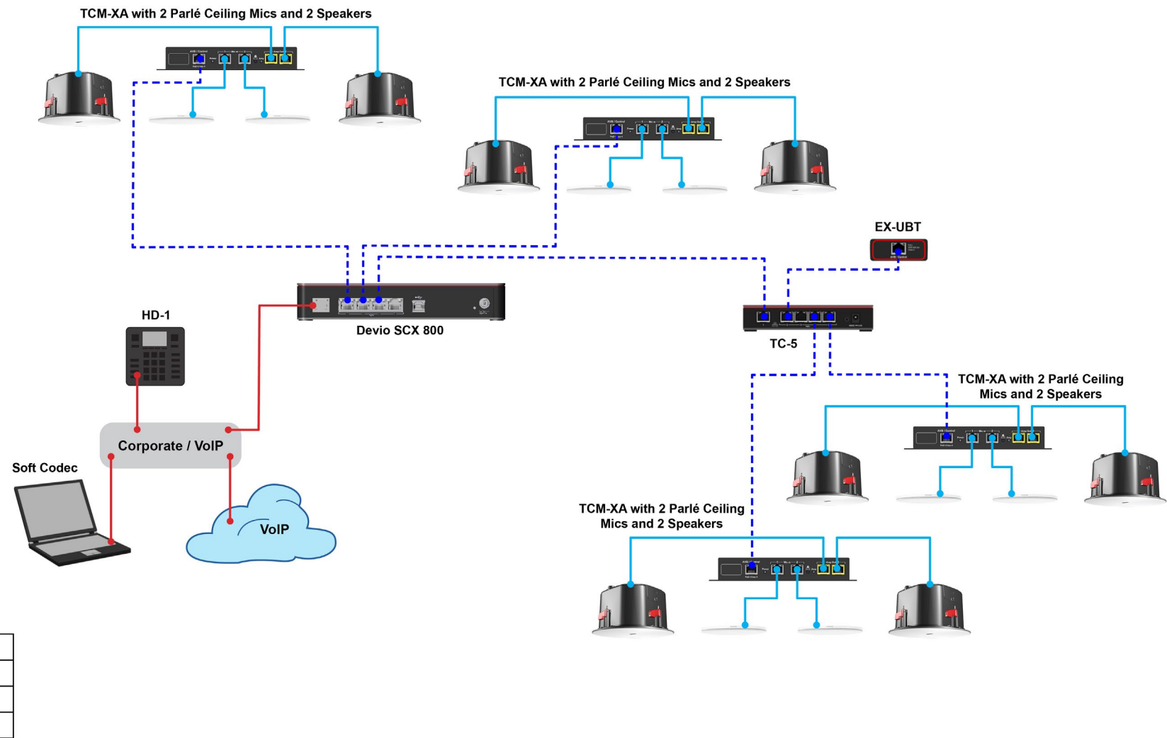
Devio SCX 800 Large Meeting Room with Eight Ceiling Mics
