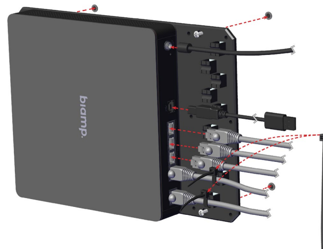
Figure 4 - Devio SCX Wall Installation with Cable Management Tray
