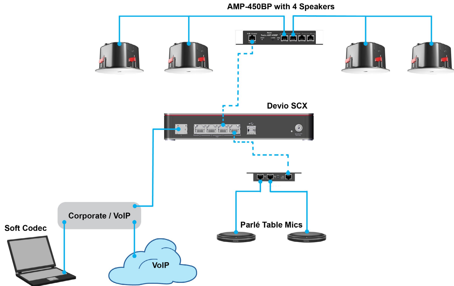
Devio SCX 400 Large Meeting Room with Two Table-Top Mics
