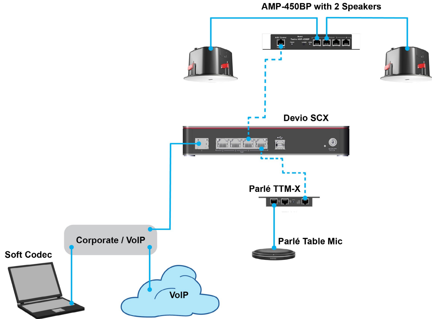
Devio SCX 400 Medium Meeting Room with One Table-Top Mic
