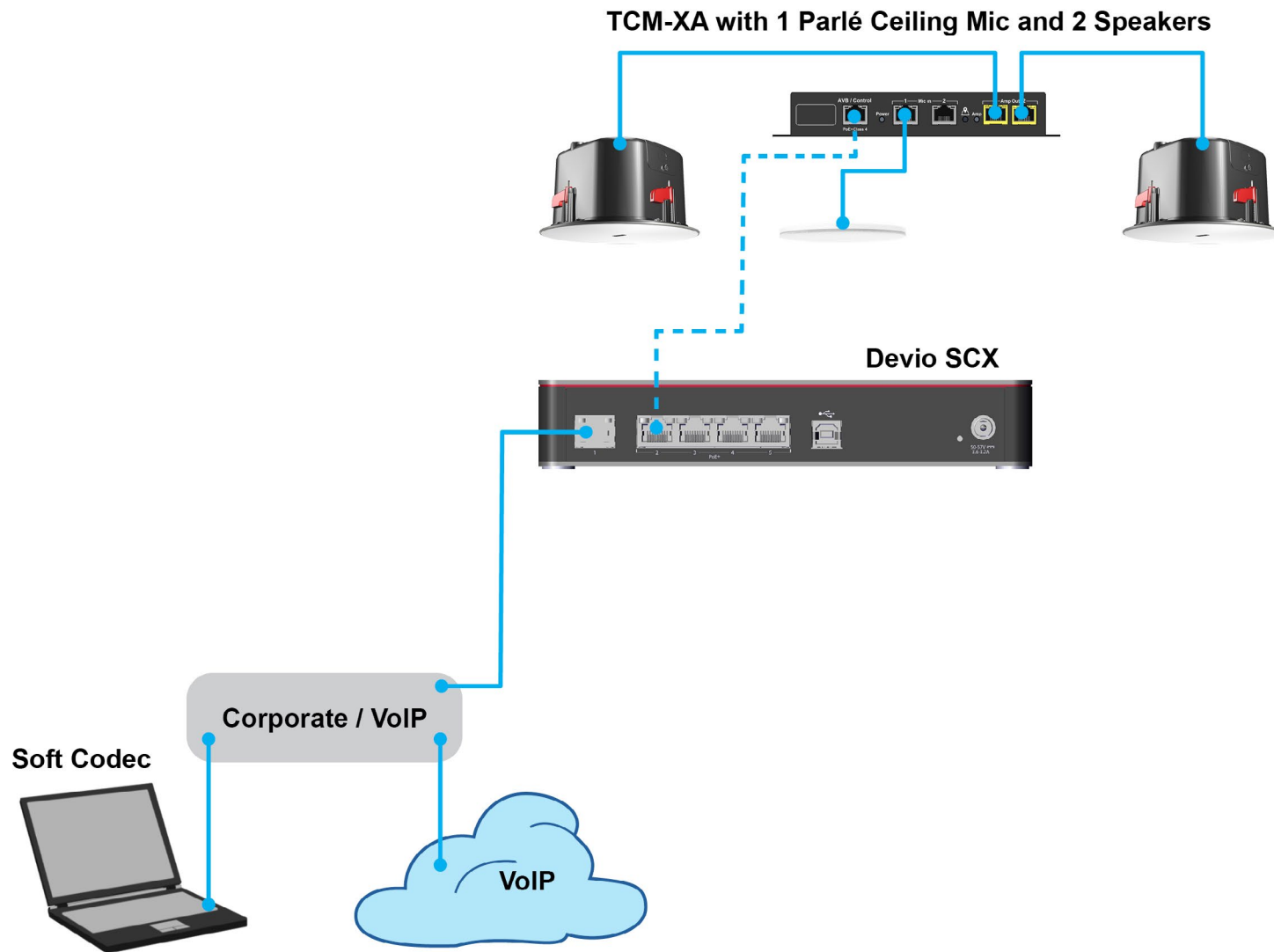
Devio SCX 400 Medium Meeting Room with One Ceiling Mic
