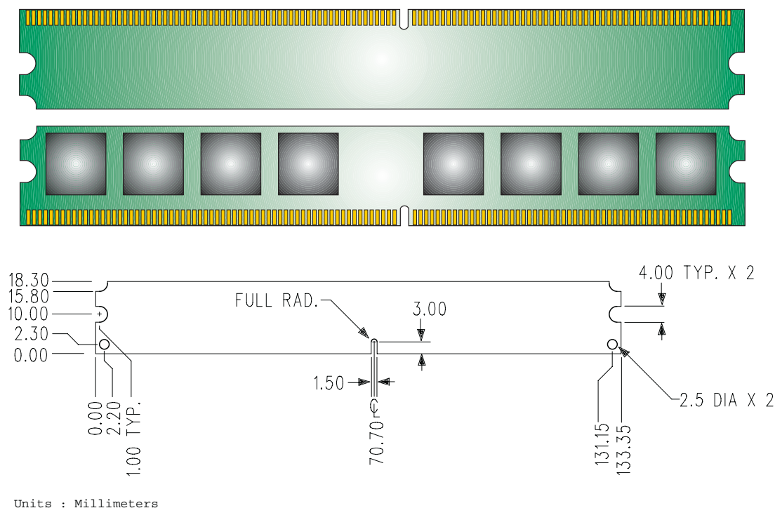
Figure 1: KVR667D2N5K2/2G 240-Pin DIMM Kit
