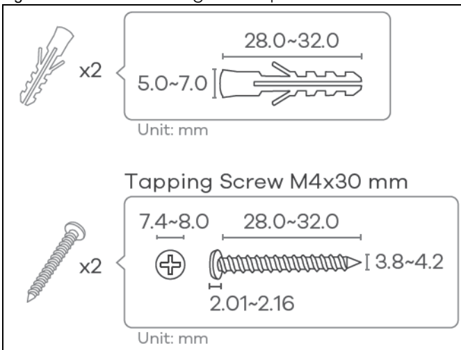
Figure 28 Wall Mounting Screw Specifications
