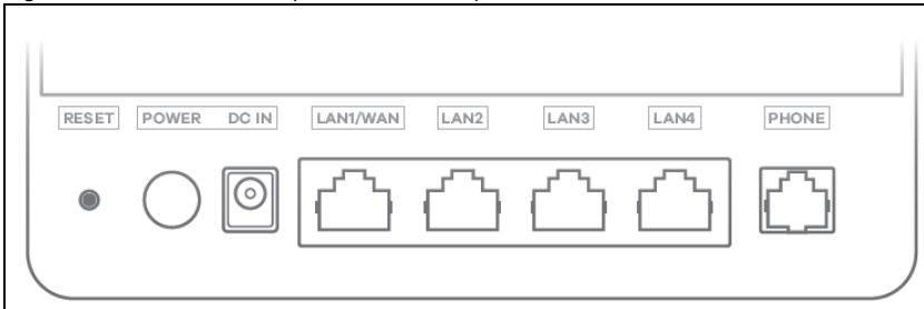
Figure 16 Side Panel (LTE3316-M604)
