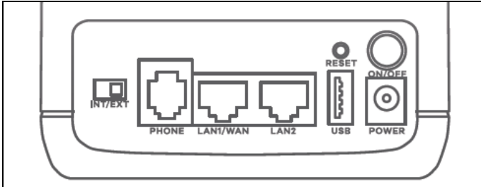
Figure 13 Rear Panel (LTE5388-M804 / LTE5398-M904)
