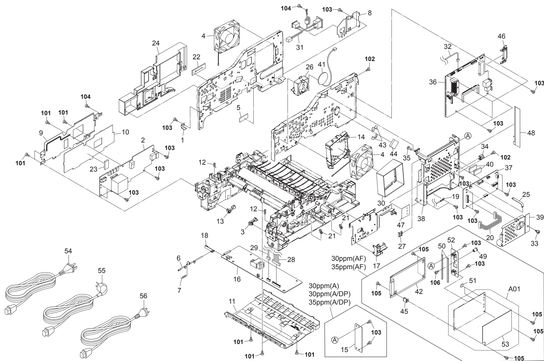
FIG. 12 Electrical Components(30ppm(A),30ppm(A/DP),30ppm(AF),35ppm(A/DP),35ppm(AF))
