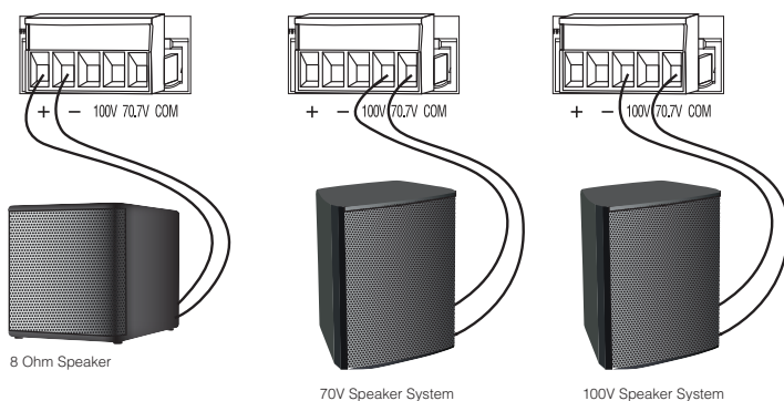
Figure 2.5 Output Wiring
