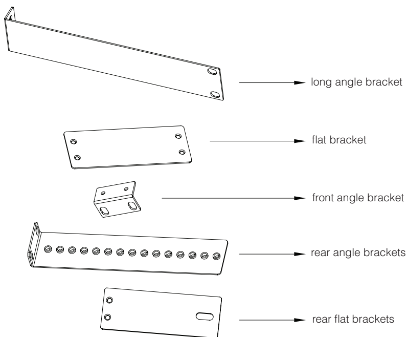
Figure 2.2.2 Mounting Kit
