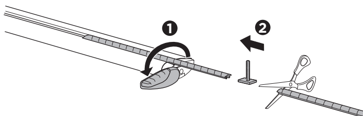
THULE WingBar
