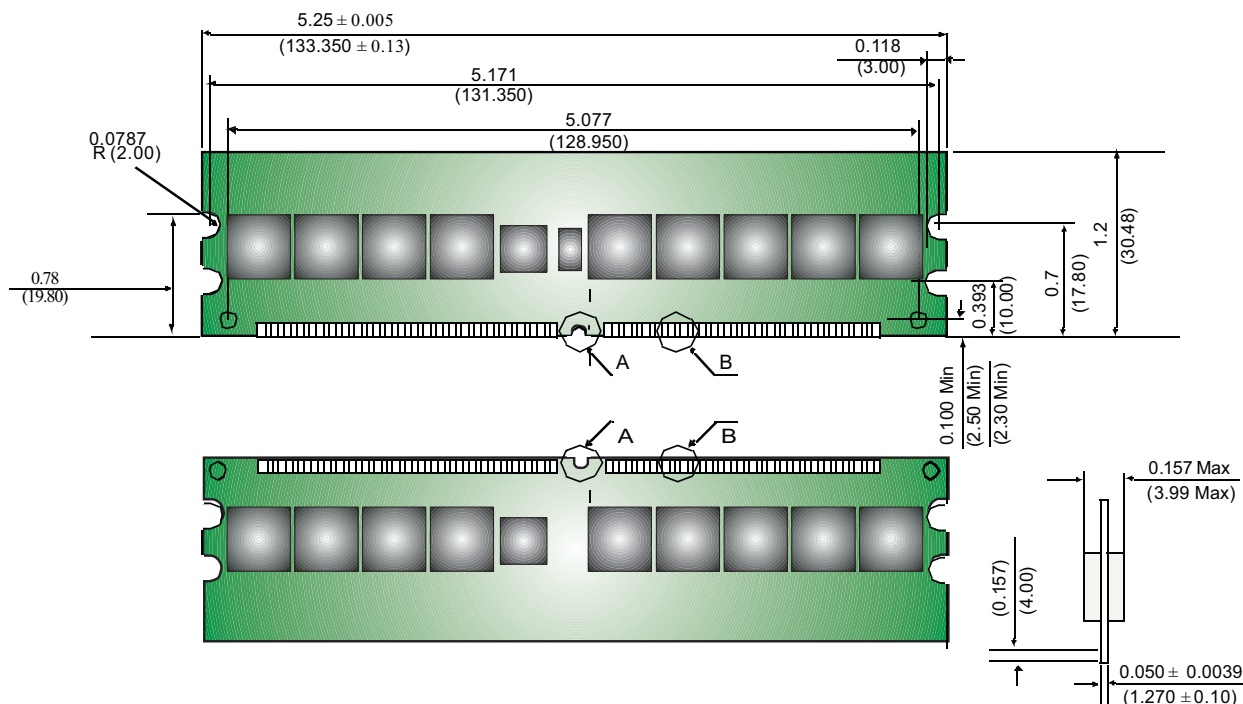
Figure 1: KVR400S4R3A/1G 184-Pin DIMM
