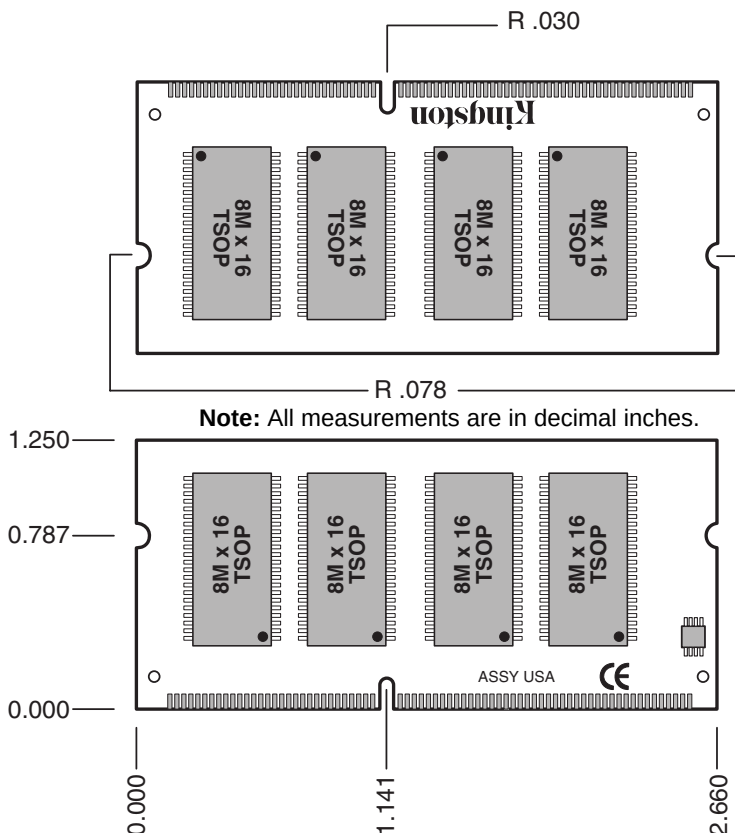
Figure 1: KVR133X64SC3/128 144-Pin SDRAM Module
