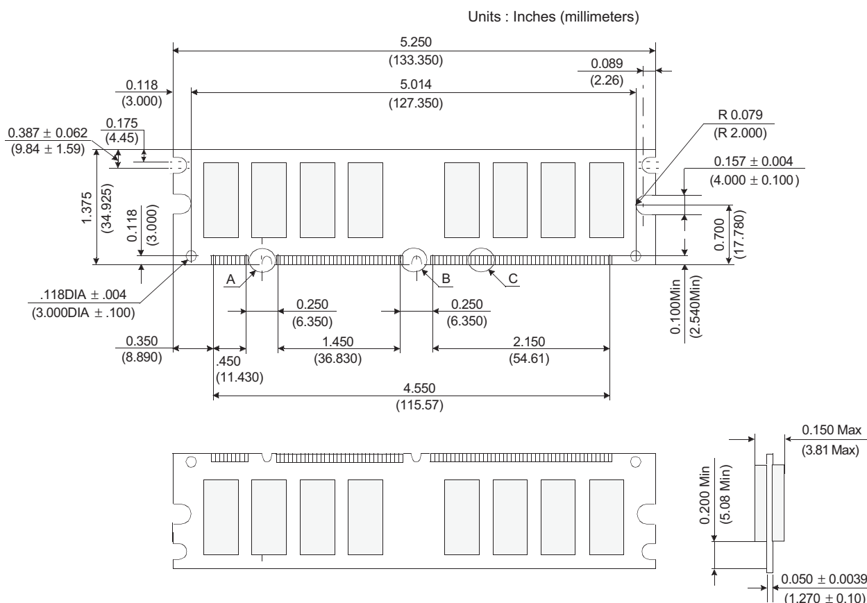
Figure 1: KVR133X64C3/512 168-Pin SDRAM Module
