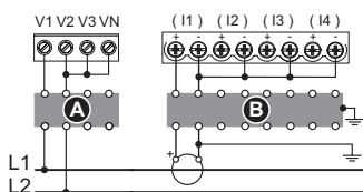
1PH2W LL
