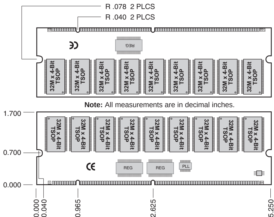
Figure 1: KVR133X72RC3/256-IS 168-Pin SDRAM Module
