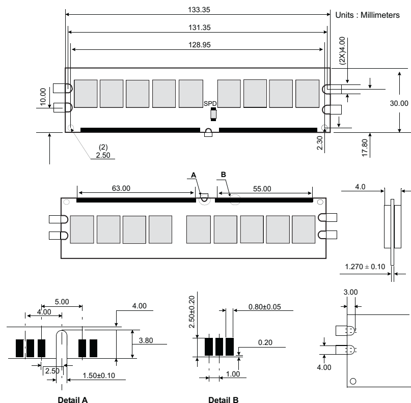
Figure 1: KVR533D2E4/1GI 240-Pin DIMM
