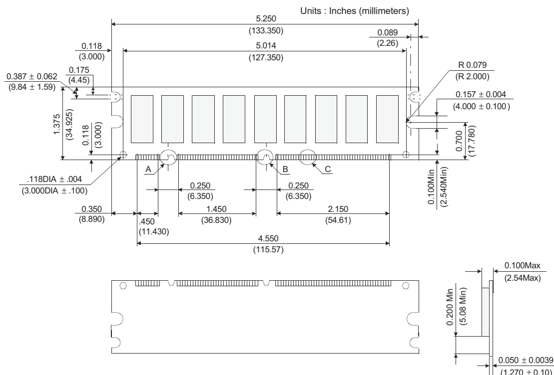
Figure 1: KVR100X72C2/128 168-Pin SDRAM Module
