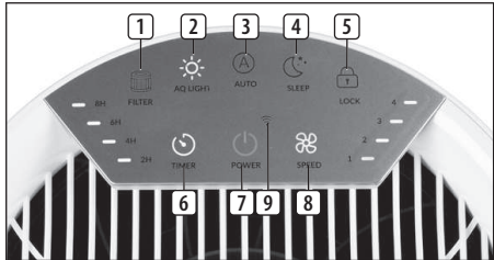
CONTROL PANEL
