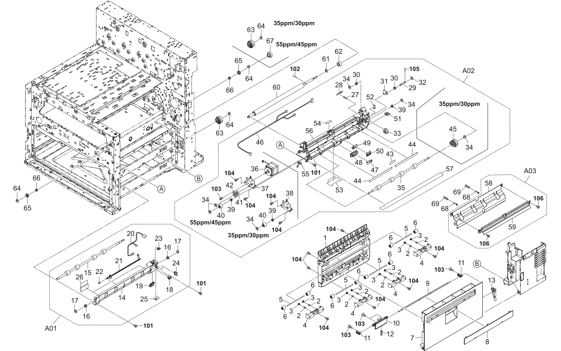
FIG. 8 Paper Feed Section 2
