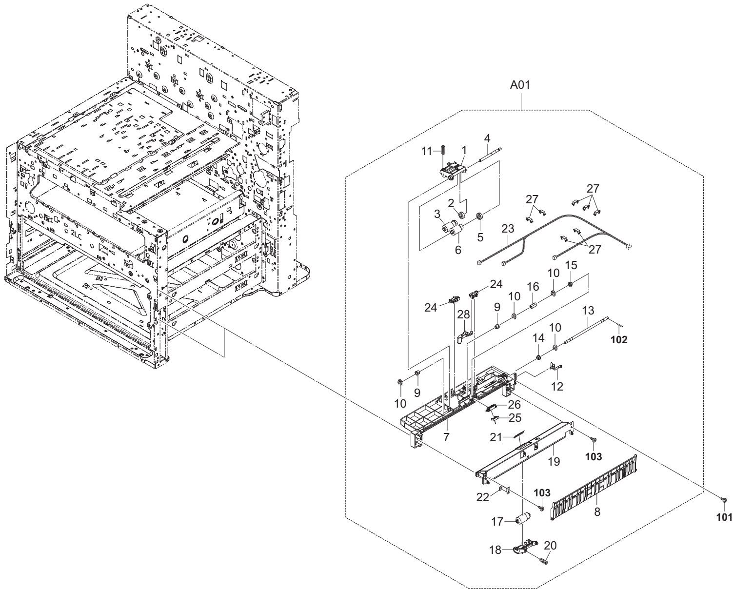
FIG. 7 Paper Feed Section 1 (35ppm/30ppm)
