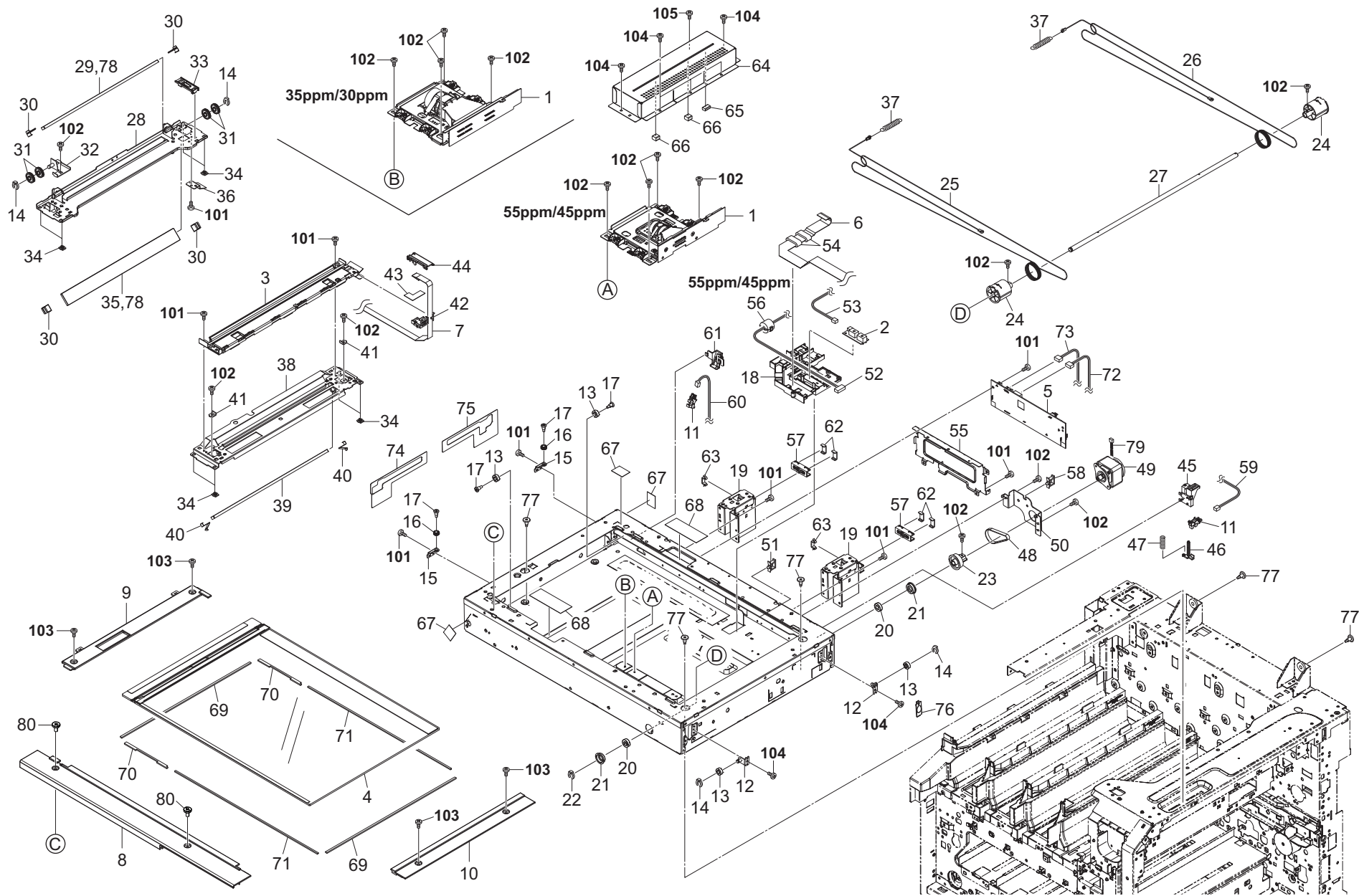
FIG. 12 Scanner Section
