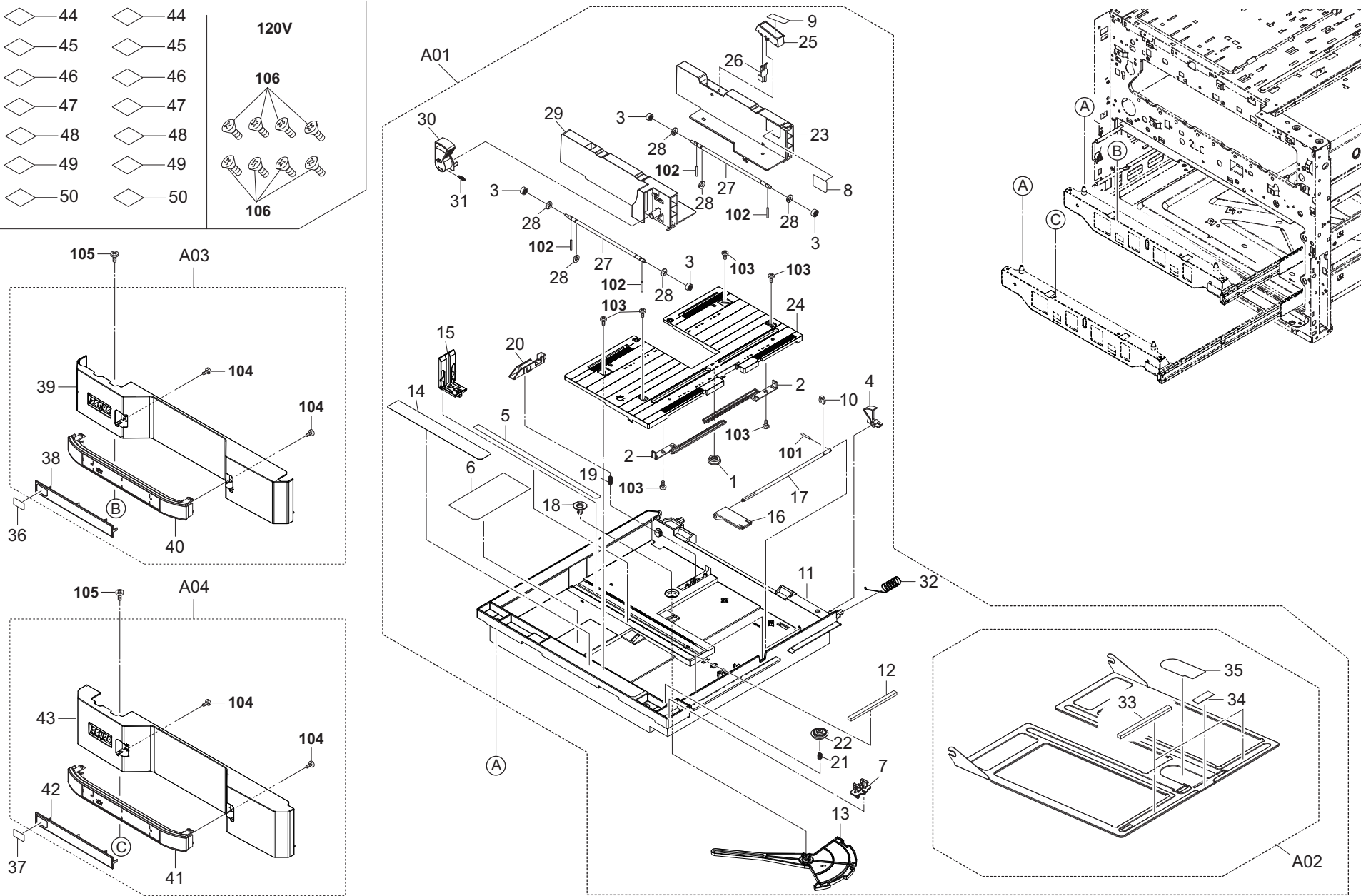
FIG. 6 Paper Cassettes
