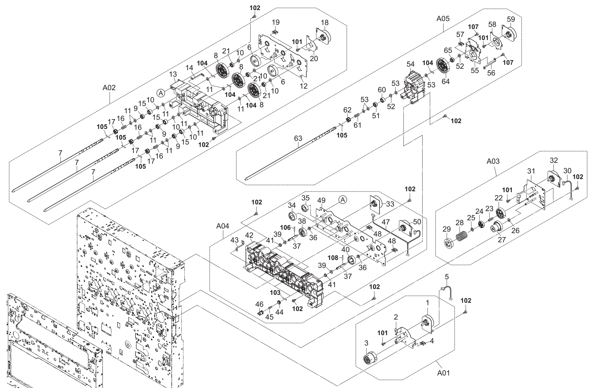
FIG. 19 Drive Section 1 (35ppm/30ppm)
