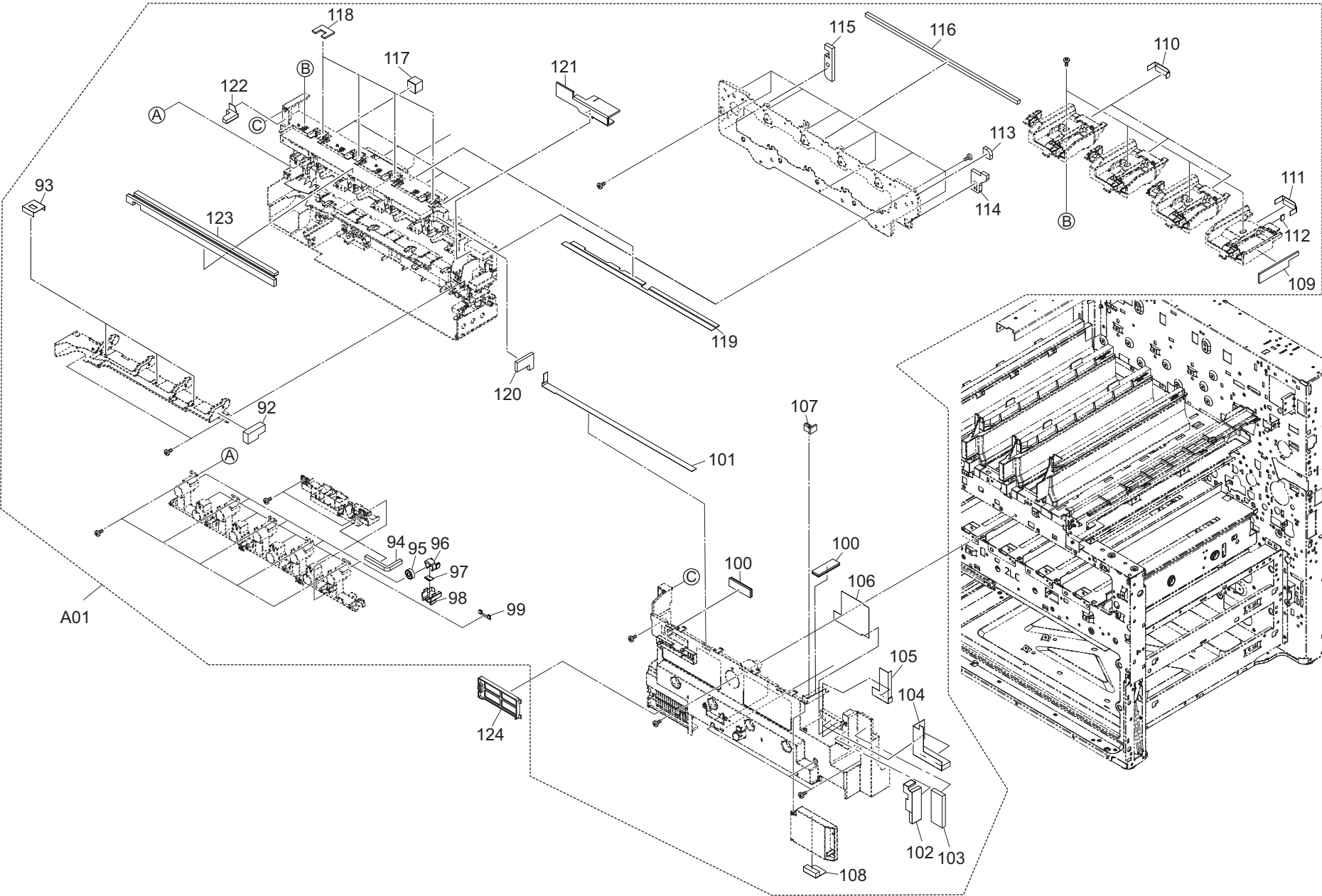
FIG. 15 Inner Section 1-2
