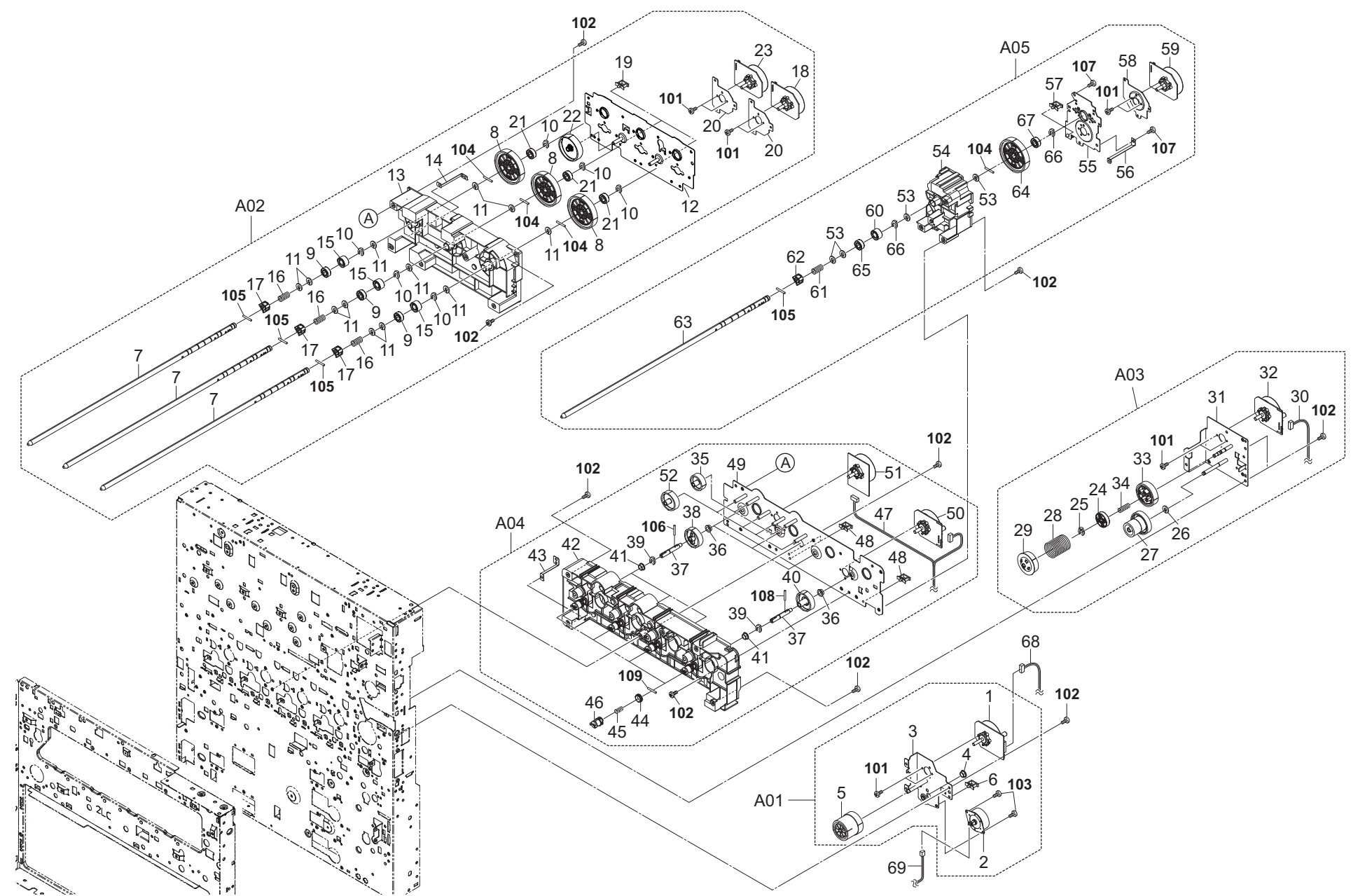
FIG. 19 Drive Section 1 (55ppm/45ppm)
