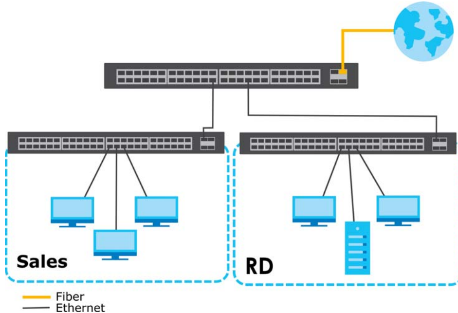
Figure 4 Bridging / Fiber Uplink Example Application
