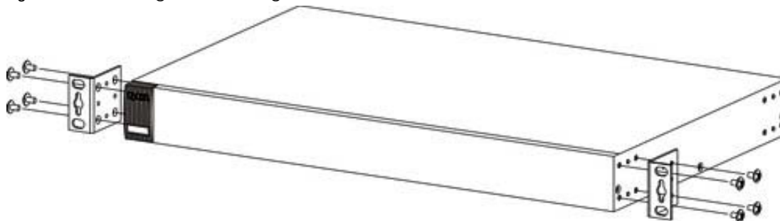
Figure 8 Attaching the Mounting Brackets
