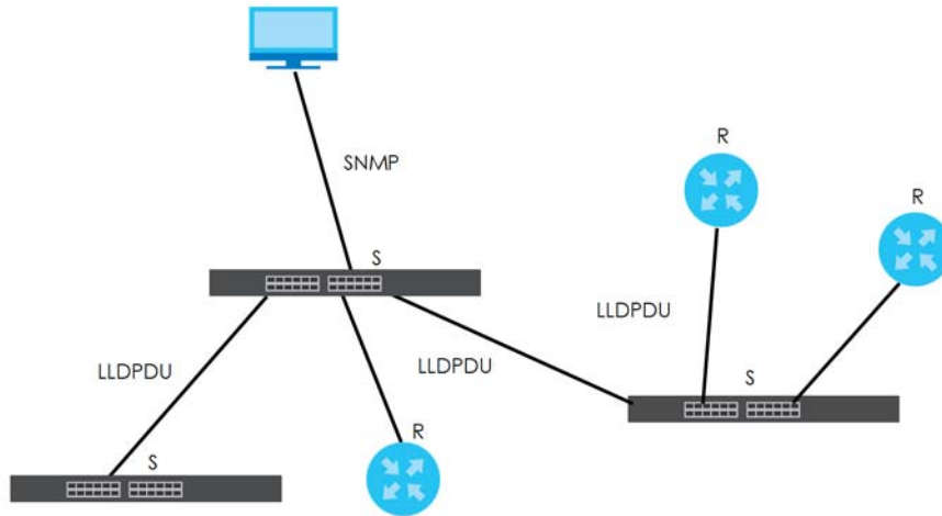
Figure 166 LLDP Overview
