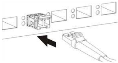
Figure 13 Connecting the Fiber Optic Cables
