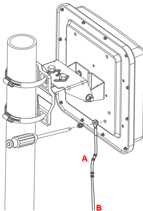
Figure 12 Grounding Example
