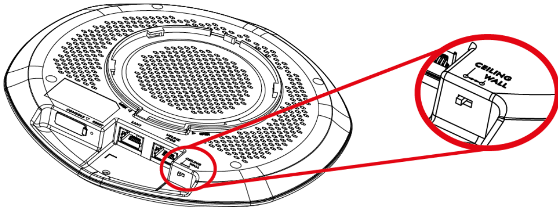
Figure 123 WAC6103D-I Physical Antenna Switch
