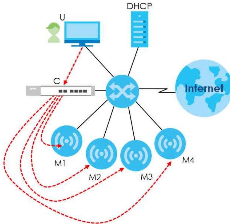
Figure 40 CAPWAP Network Example
