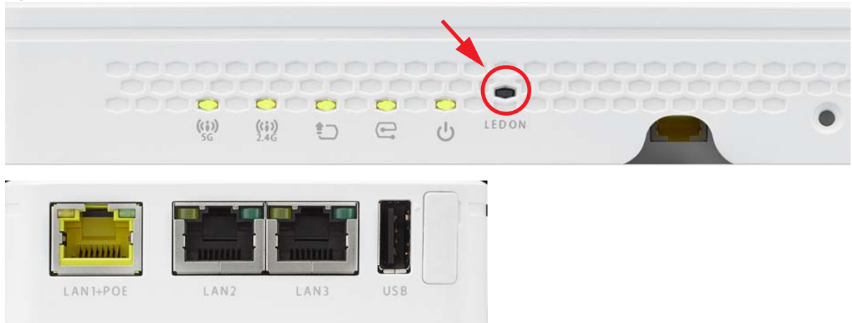
Figure 8 WAC5302D-S LEDs
