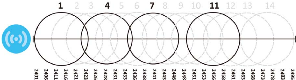
Figure 57 An Example Four-Channel Deployment
