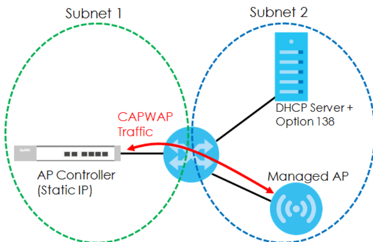
Figure 41 CAPWAP and DHCP Option 138
