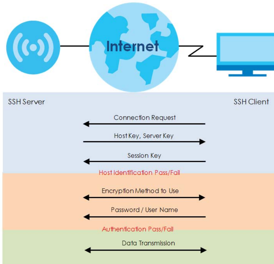
Figure 100 How SSH v1 Works Example
