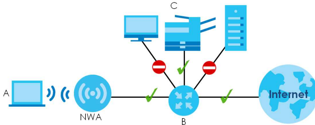
Figure 74 Layer-2 Isolation Application
