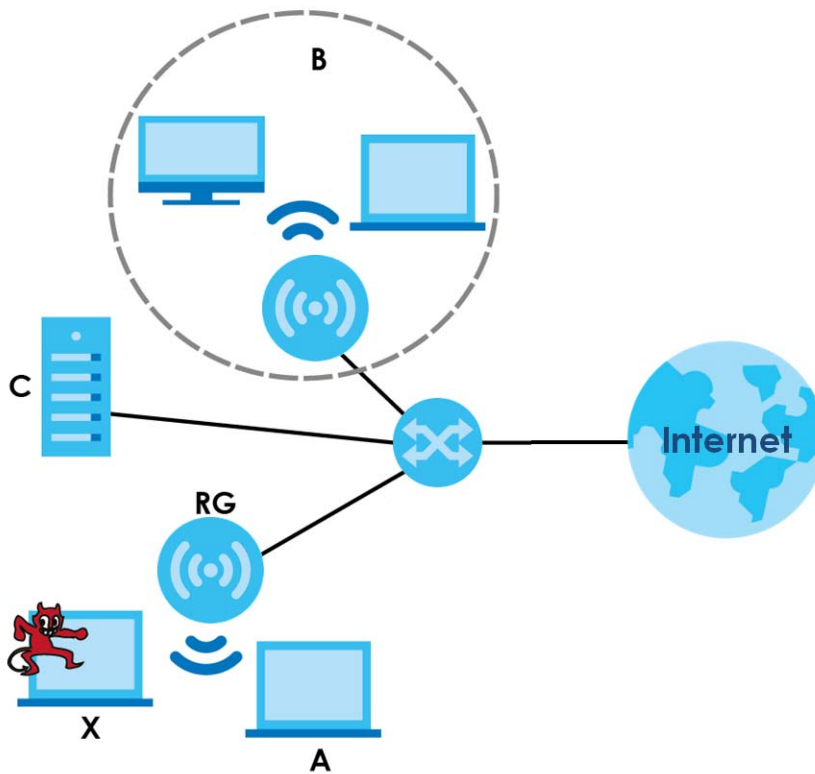
Figure 79 Rogue AP Example
