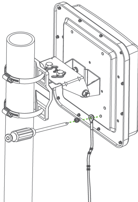
Figure 10 Grounding Example
