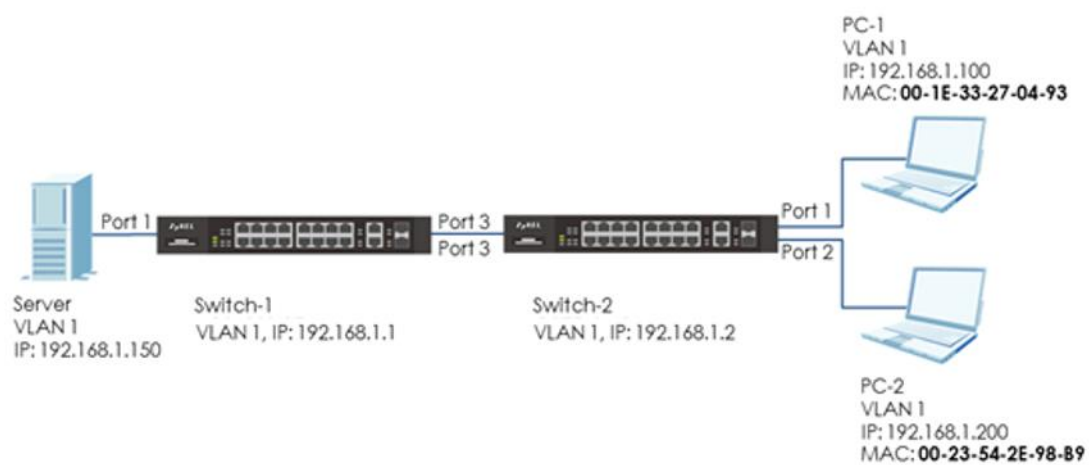
Figure 20 Configure MAC filter to block unwanted traffic
