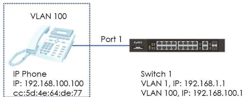
Figure 24 Configure Voice VLAN to separate VOIP traffic from data traffic
