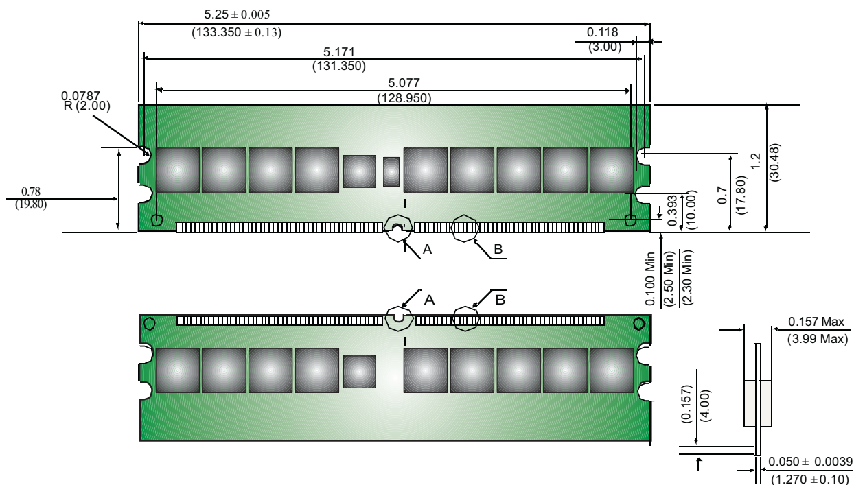
Figure 1: KVR400S4R3A/512 184-Pin DIMM
