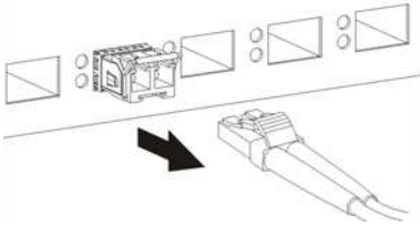
Figure 16 Removing the Fiber Optic Cables
