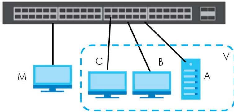
Figure 49 Tutorial: DHCP Snooping Tutorial Overview
