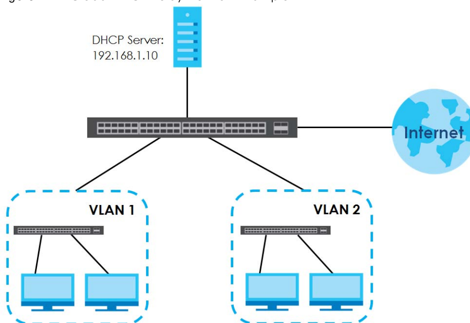
Figure 172 Global DHCP Relay Network Example
