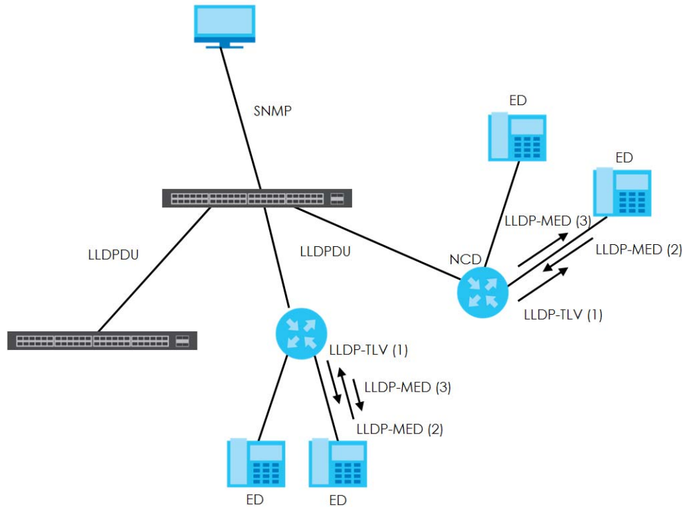
Figure 145 LLDP-MED Overview
