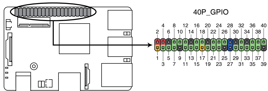
Tinker Board 2 / 2S 40-pins GPIO header
