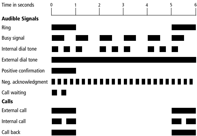
Handset and ring patterns on BlueFRITZ! AP-X extension telephones
