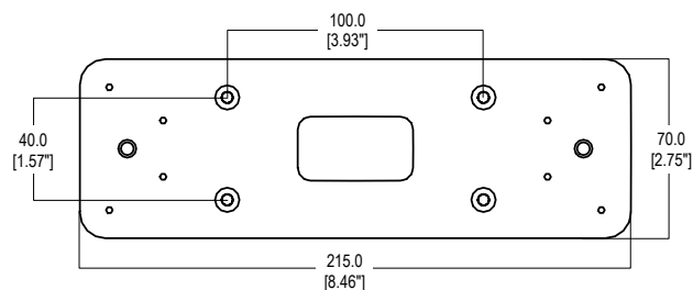
WALL PLATE
