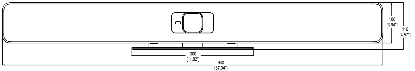
FRONT
