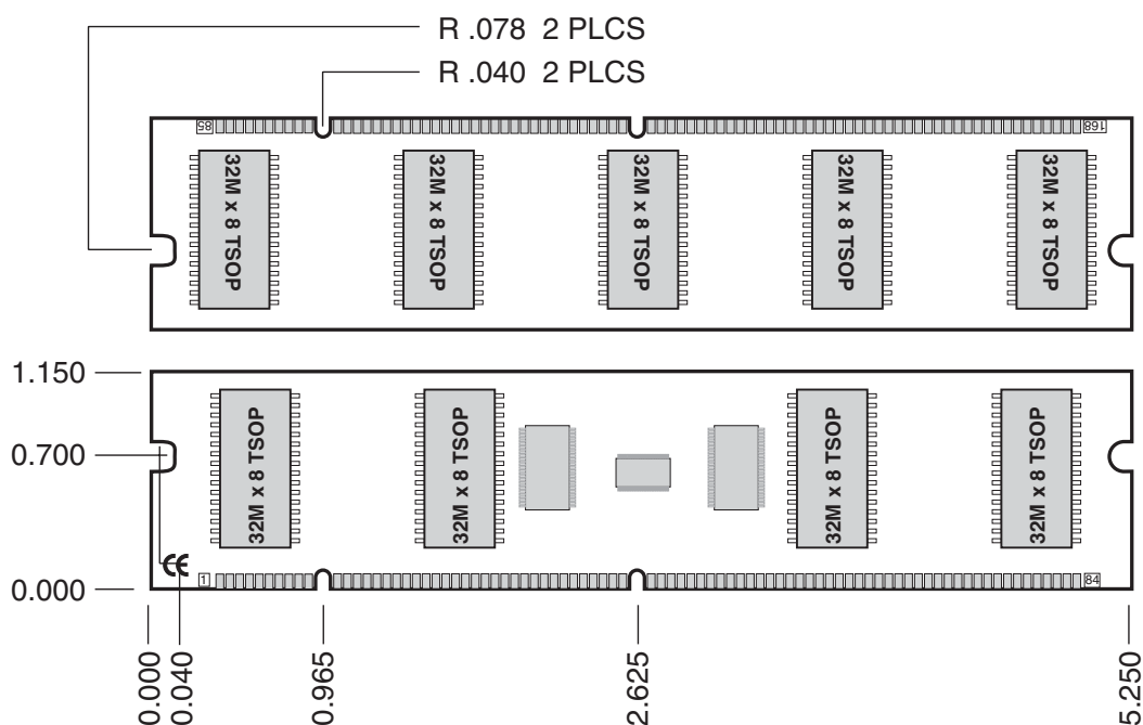
Figure 1: KVR133X72RC3L/256 168-Pin SDRAM Module
