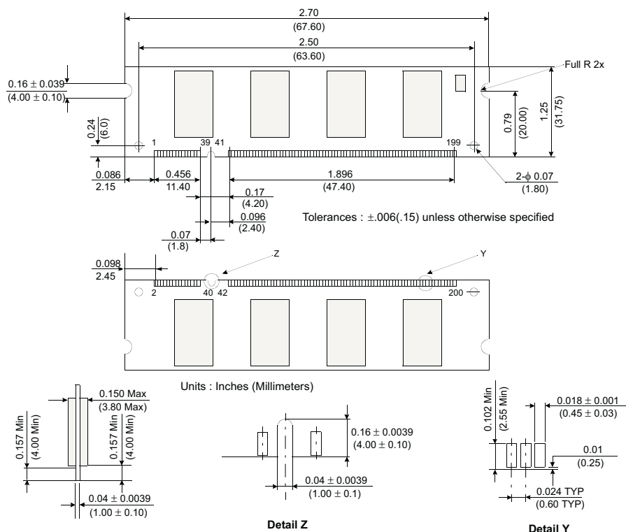
Figure 1: KVR266X64SC25/256 200-Pin DDR SDRAM Module
