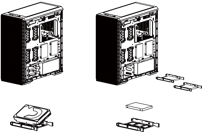
3.5" HDD Installation
