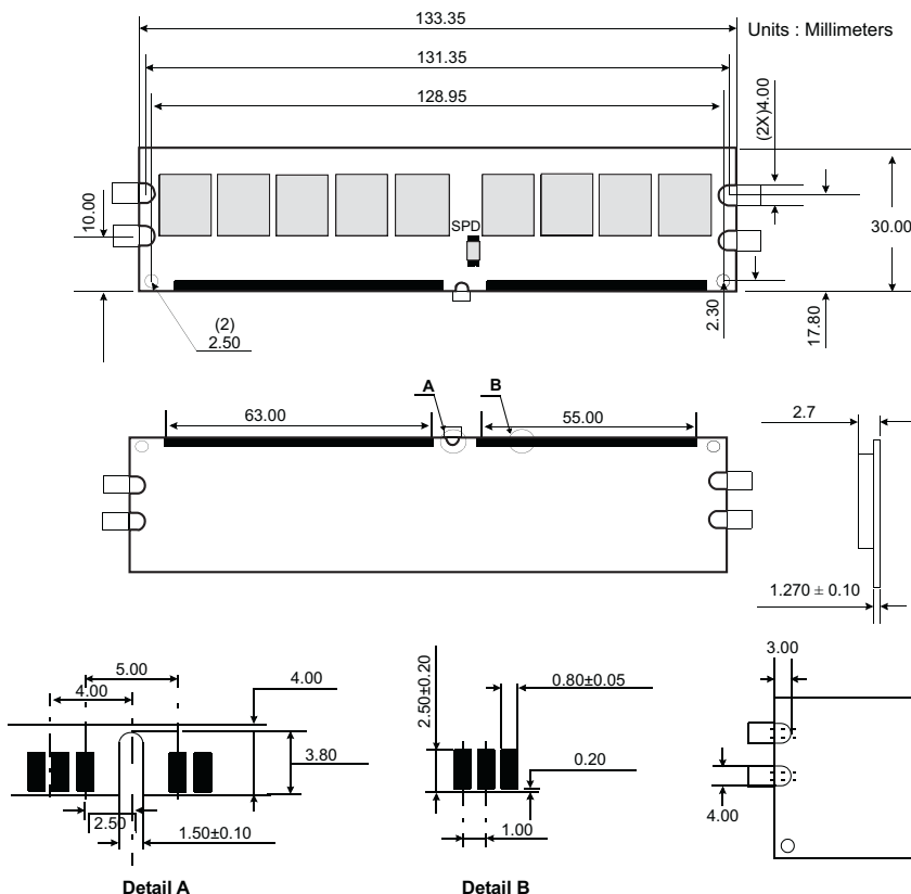
Figure 1: KVR533D2E4/256 240-Pin DIMM
